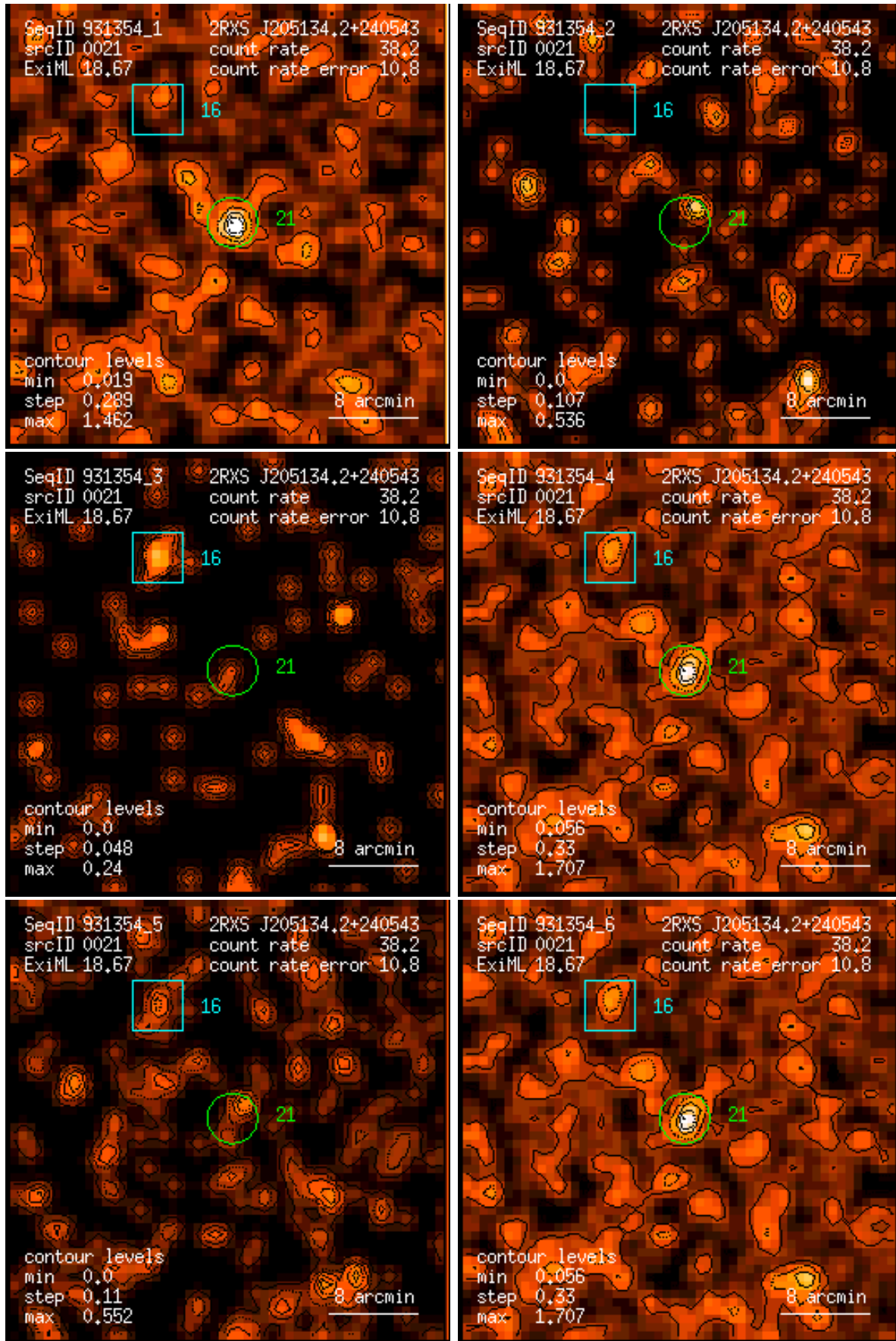
Figure 21: RASS 931354: detection 0021: band rate images, Gaussian filter: (1) PSPC channels 11 – 41, (2) 52 – 90, (3) 91 – 201, (4) 11 – 235, (5) 52 – 201, (6) 11 – 201. Broad band rates in counts/ks. Band rate contour levels in counts/ks/arcmin 2 .
