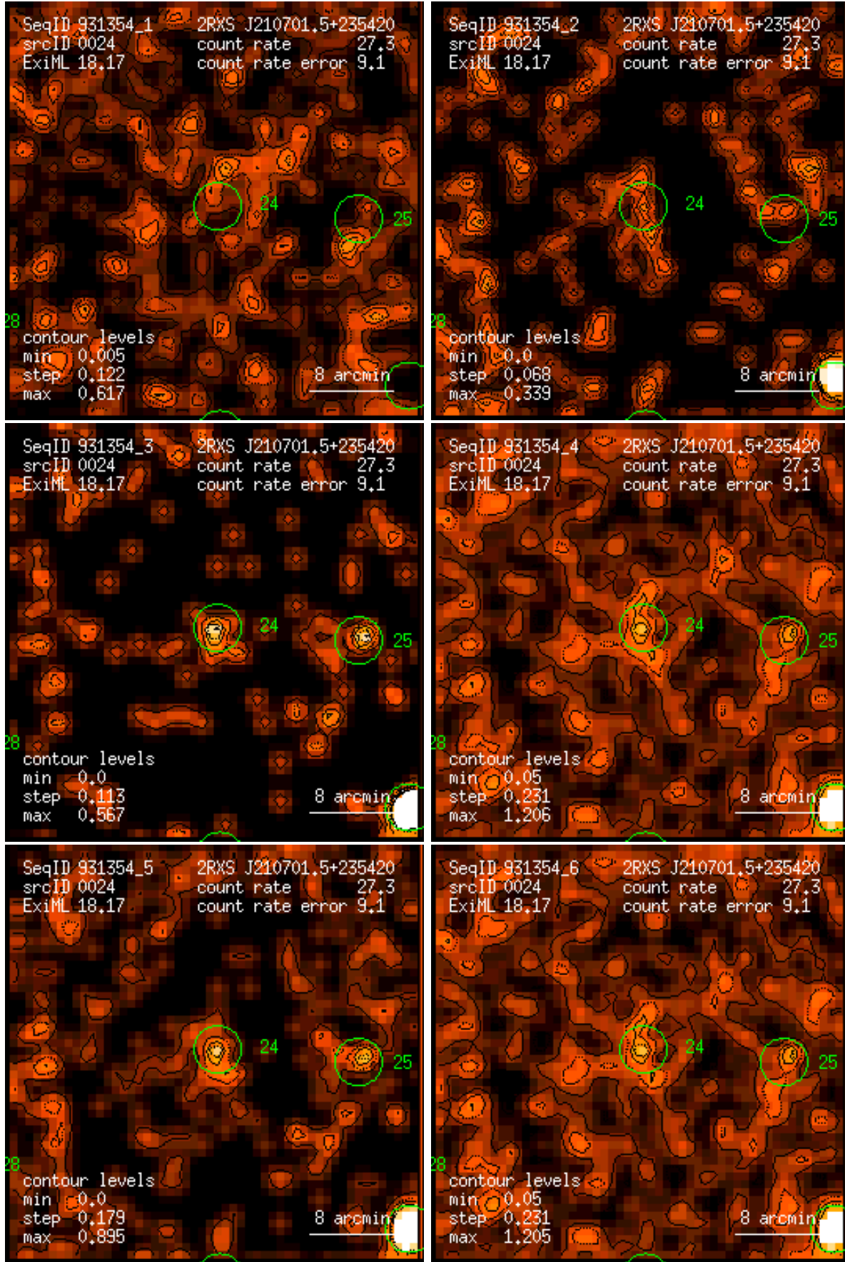
Figure 24: RASS 931354: detection 0024: band rate images, Gaussian filter: (1) PSPC channels 11 – 41, (2) 52 – 90, (3) 91 – 201, (4) 11 – 235, (5) 52 – 201, (6) 11 – 201. Broad band rates in counts/ks. Band rate contour levels in counts/ks/arcmin 2 .
