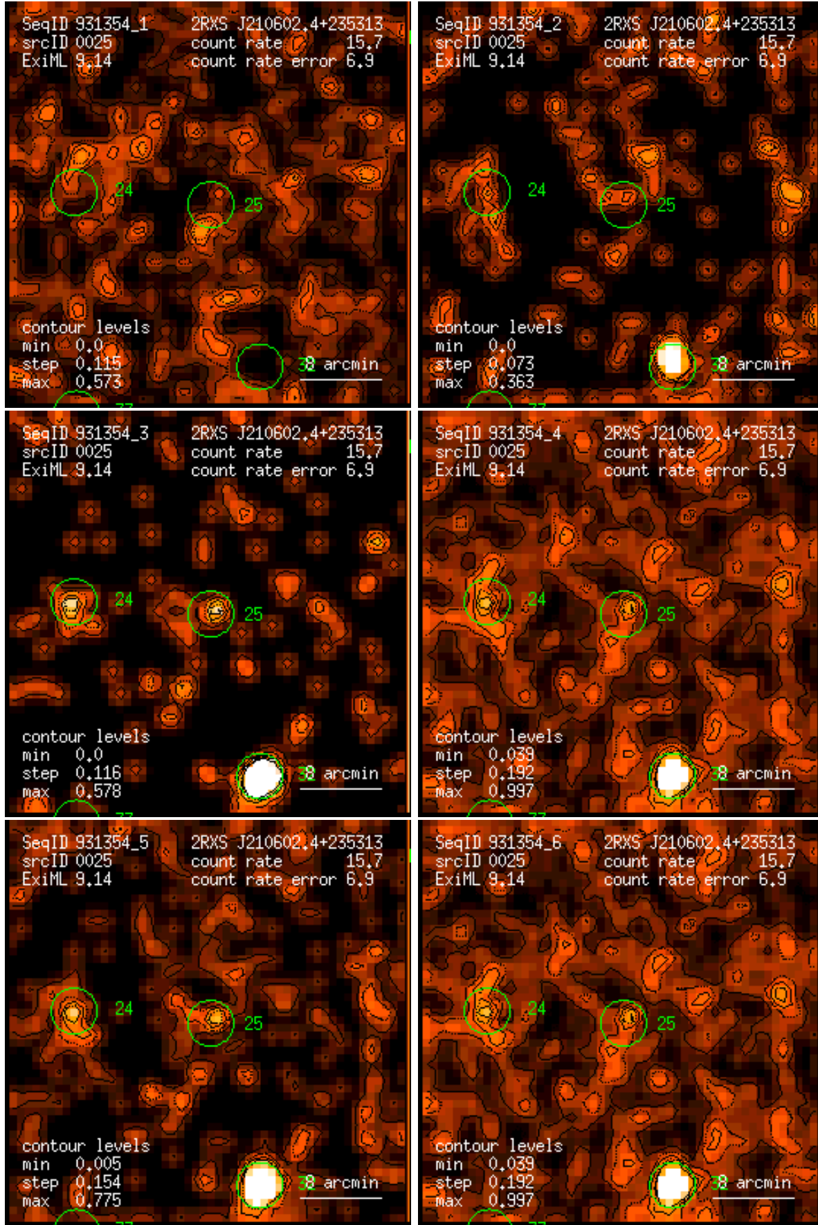
Figure 25: RASS 931354: detection 0025: band rate images, Gaussian filter: (1) PSPC channels 11 – 41, (2) 52 – 90, (3) 91 – 201, (4) 11 – 235, (5) 52 – 201, (6) 11 – 201. Broad band rates in counts/ks. Band rate contour levels in counts/ks/arcmin 2 .
