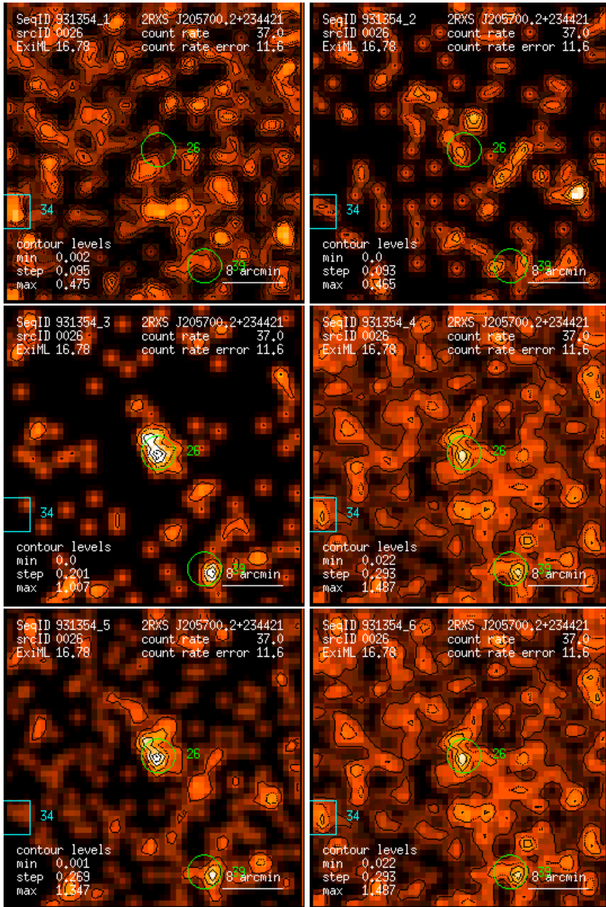
Figure 26: RASS 931354: detection 0026: band rate images, Gaussian filter: (1) PSPC channels 11 – 41, (2) 52 – 90, (3) 91 – 201, (4) 11 – 235, (5) 52 – 201, (6) 11 – 201. Broad band rates in counts/ks. Band rate contour levels in counts/ks/arcmin 2 .
