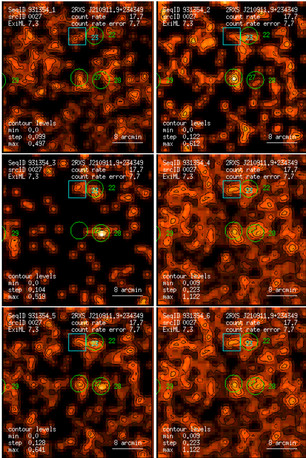
Figure 27: RASS 931354: detection 0027: band rate images, Gaussian filter: (1) PSPC channels 11 – 41, (2) 52 – 90, (3) 91 – 201, (4) 11 – 235, (5) 52 – 201, (6) 11 – 201. Broad band rates in counts/ks. Band rate contour levels in counts/ks/arcmin 2 .
