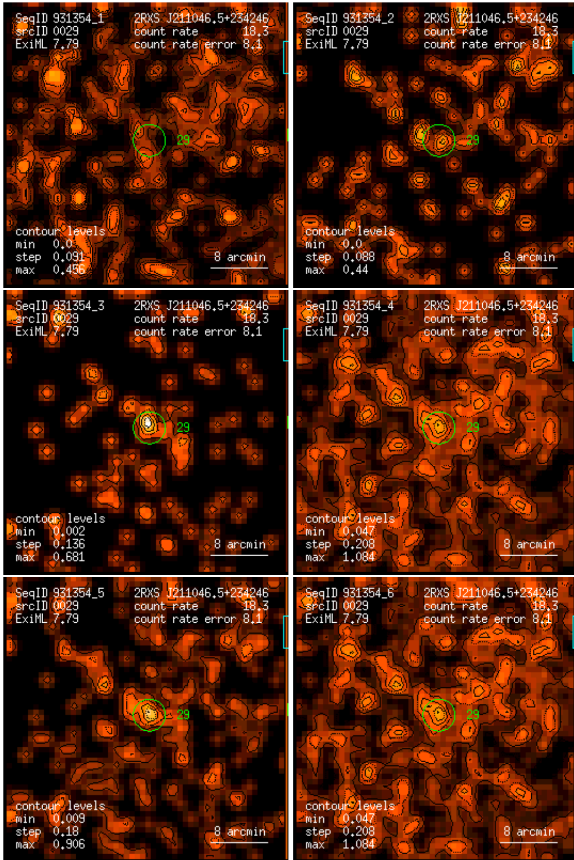
Figure 29: RASS 931354: detection 0029: band rate images, Gaussian filter: (1) PSPC channels 11 – 41, (2) 52 – 90, (3) 91 – 201, (4) 11 – 235, (5) 52 – 201, (6) 11 – 201. Broad band rates in counts/ks. Band rate contour levels in counts/ks/arcmin 2 .
