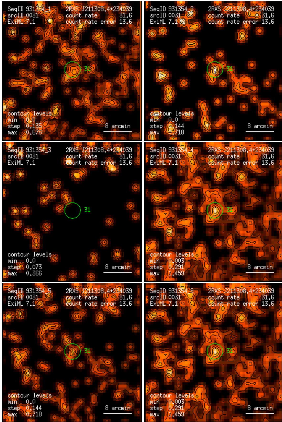
Figure 31: RASS 931354: detection 0031: band rate images, Gaussian filter: (1) PSPC channels 11 – 41, (2) 52 – 90, (3) 91 – 201, (4) 11 – 235, (5) 52 – 201, (6) 11 – 201. Broad band rates in counts/ks. Band rate contour levels in counts/ks/arcmin 2 .
