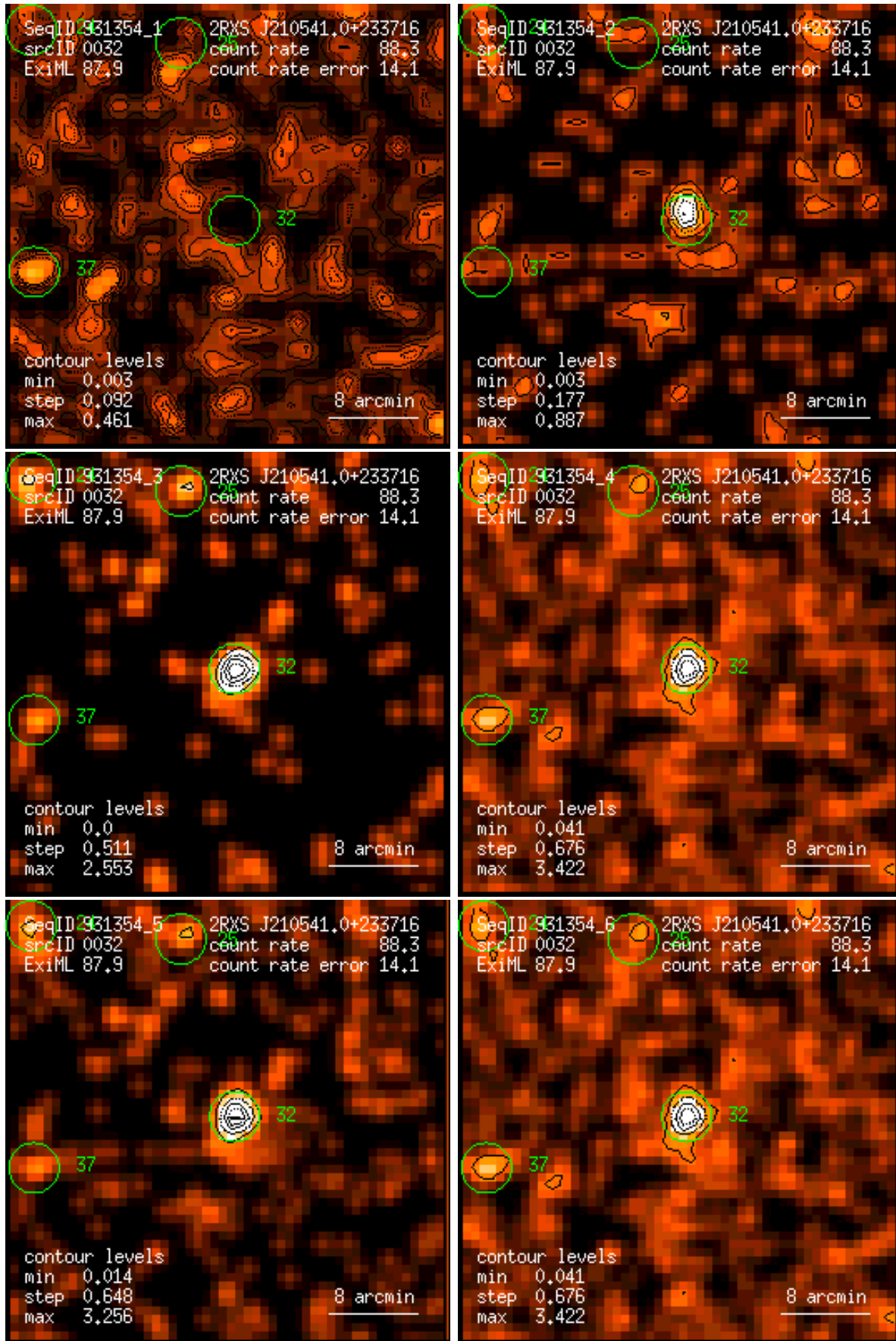
Figure 32: RASS 931354: detection 0032: band rate images, Gaussian filter: (1) PSPC channels 11 – 41, (2) 52 – 90, (3) 91 – 201, (4) 11 – 235, (5) 52 – 201, (6) 11 – 201. Broad band rates in counts/ks. Band rate contour levels in counts/ks/arcmin 2 .
