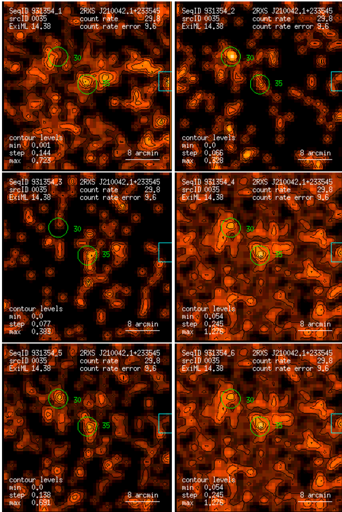
Figure 35: RASS 931354: detection 0035: band rate images, Gaussian filter: (1) PSPC channels 11 – 41, (2) 52 – 90, (3) 91 – 201, (4) 11 – 235, (5) 52 – 201, (6) 11 – 201. Broad band rates in counts/ks. Band rate contour levels in counts/ks/arcmin 2 .
