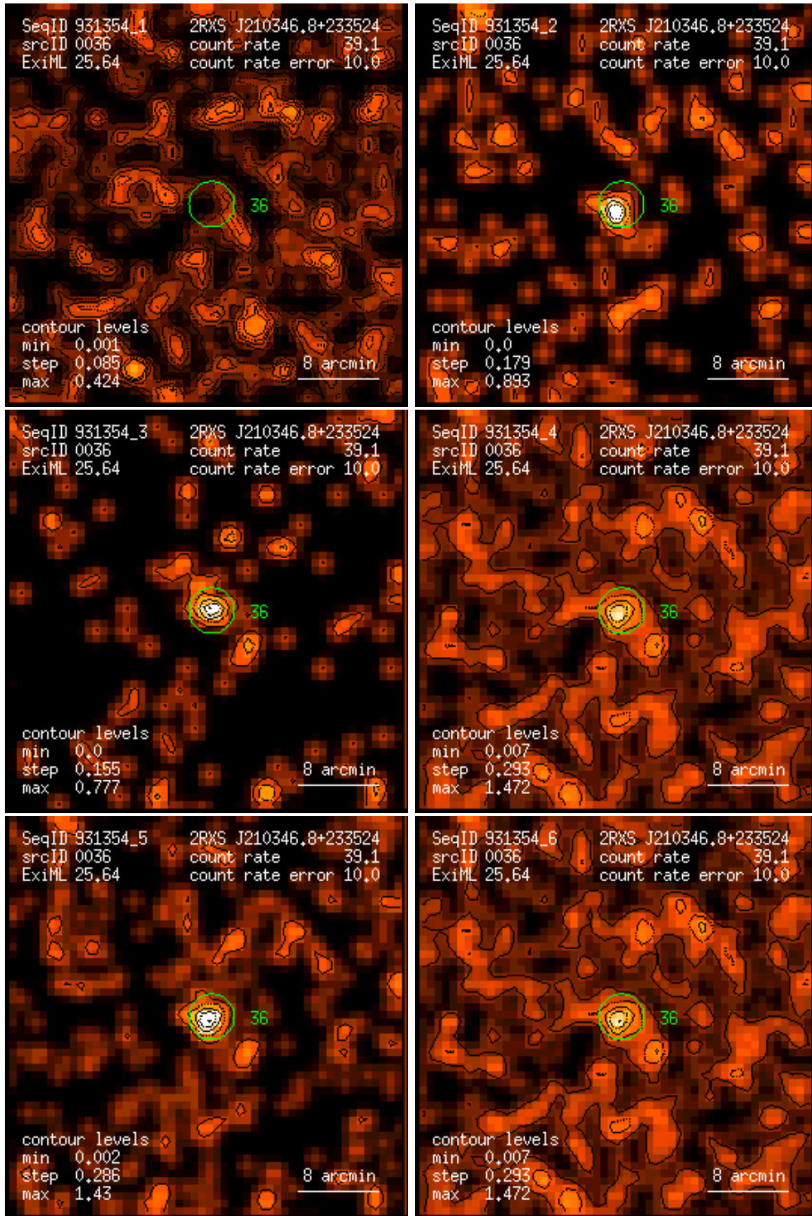
Figure 36: RASS 931354: detection 0036: band rate images, Gaussian filter: (1) PSPC channels 11 – 41, (2) 52 – 90, (3) 91 – 201, (4) 11 – 235, (5) 52 – 201, (6) 11 – 201. Broad band rates in counts/ks. Band rate contour levels in counts/ks/arcmin 2 .
