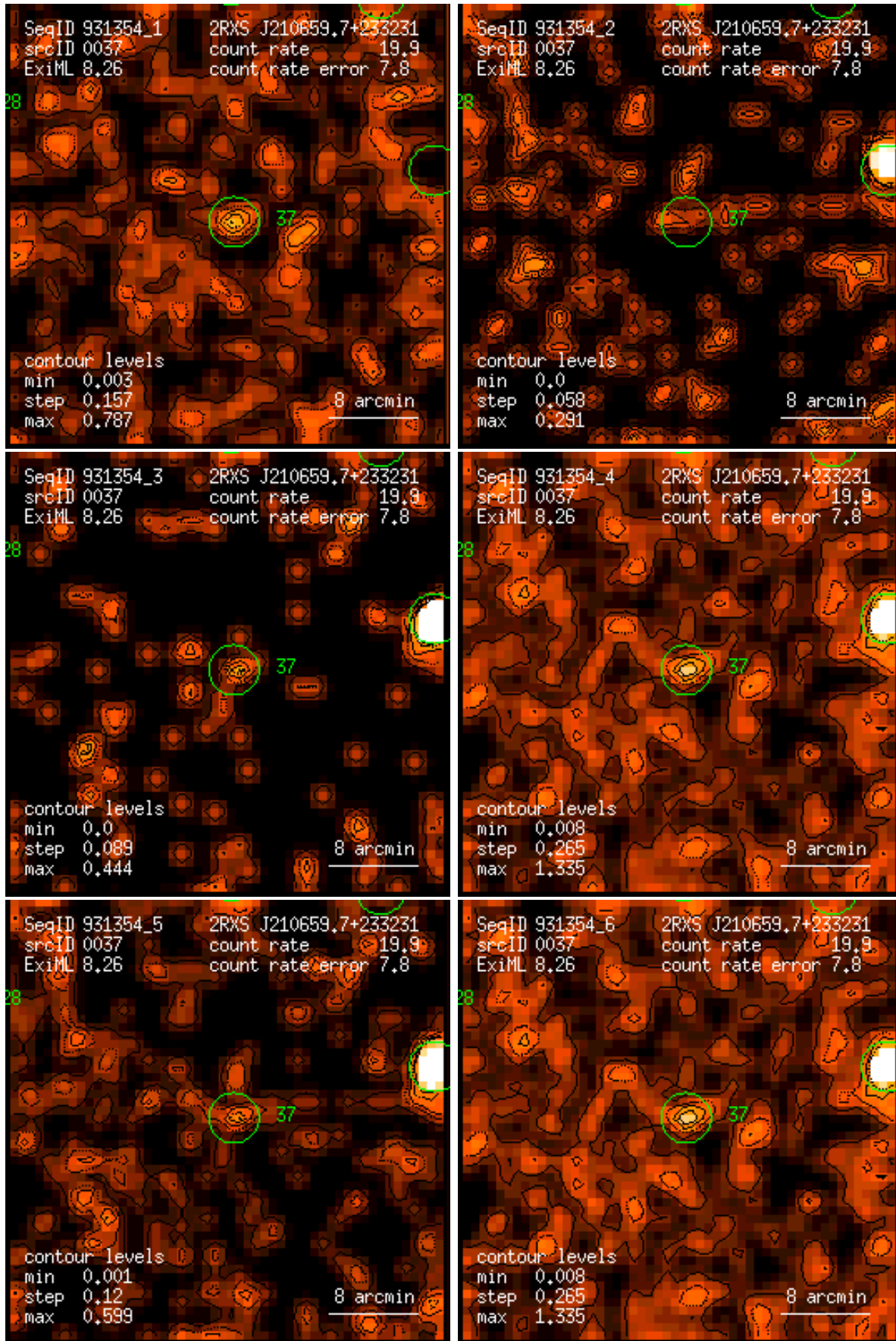
Figure 37: RASS 931354: detection 0037: band rate images, Gaussian filter: (1) PSPC channels 11 – 41, (2) 52 – 90, (3) 91 – 201, (4) 11 – 235, (5) 52 – 201, (6) 11 – 201. Broad band rates in counts/ks. Band rate contour levels in counts/ks/arcmin 2 .
