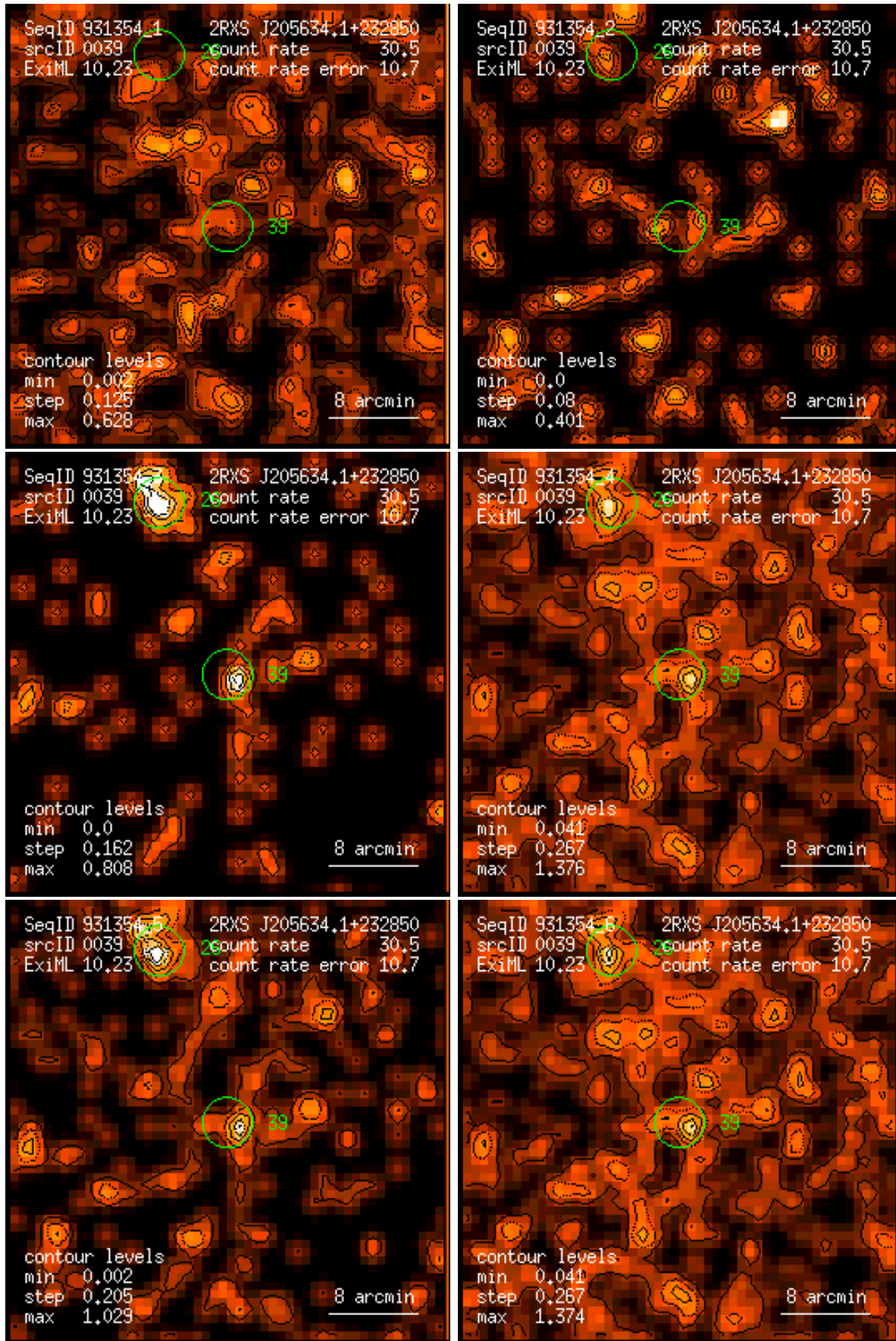
Figure 39: RASS 931354: detection 0039: band rate images, Gaussian filter: (1) PSPC channels 11 – 41, (2) 52 – 90, (3) 91 – 201, (4) 11 – 235, (5) 52 – 201, (6) 11 – 201. Broad band rates in counts/ks. Band rate contour levels in counts/ks/arcmin 2 .
