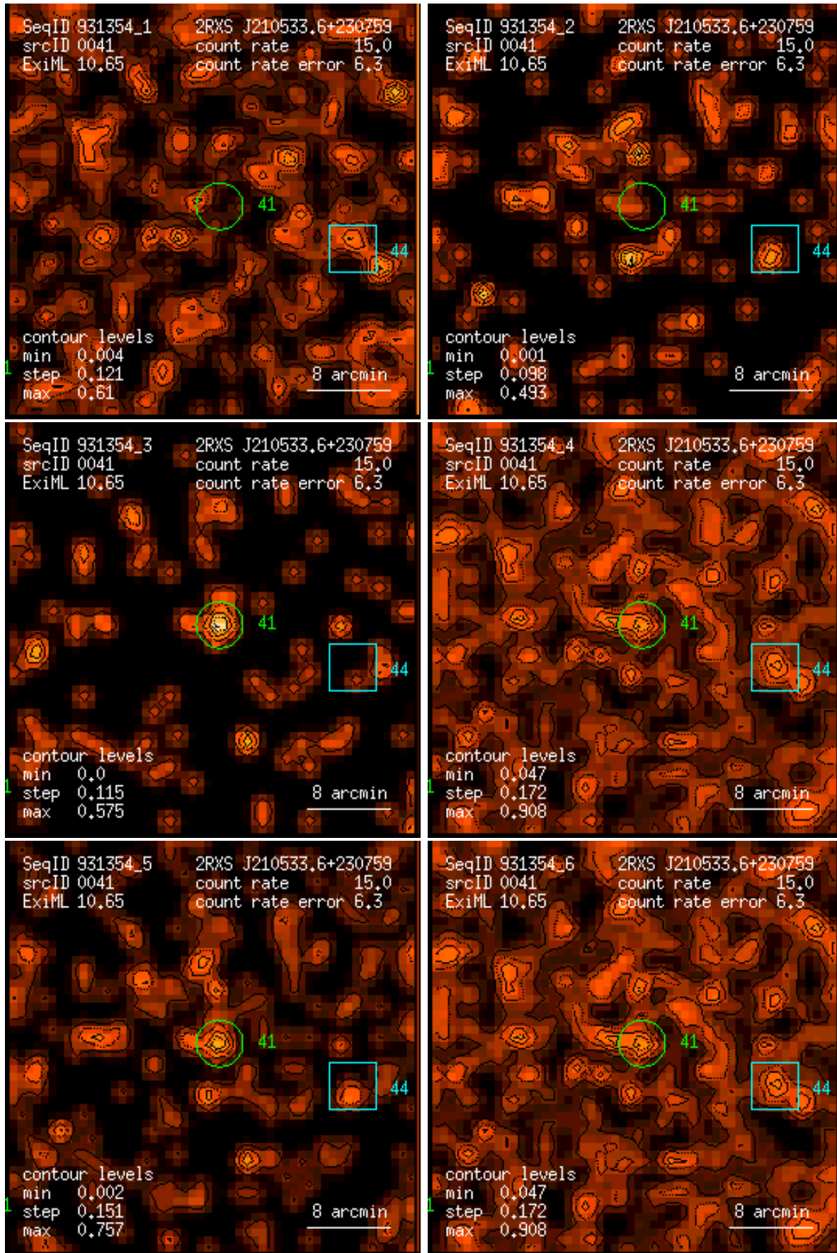
Figure 41: RASS 931354: detection 0041: band rate images, Gaussian filter: (1) PSPC channels 11 – 41, (2) 52 – 90, (3) 91 – 201, (4) 11 – 235, (5) 52 – 201, (6) 11 – 201. Broad band rates in counts/ks. Band rate contour levels in counts/ks/arcmin 2 .
