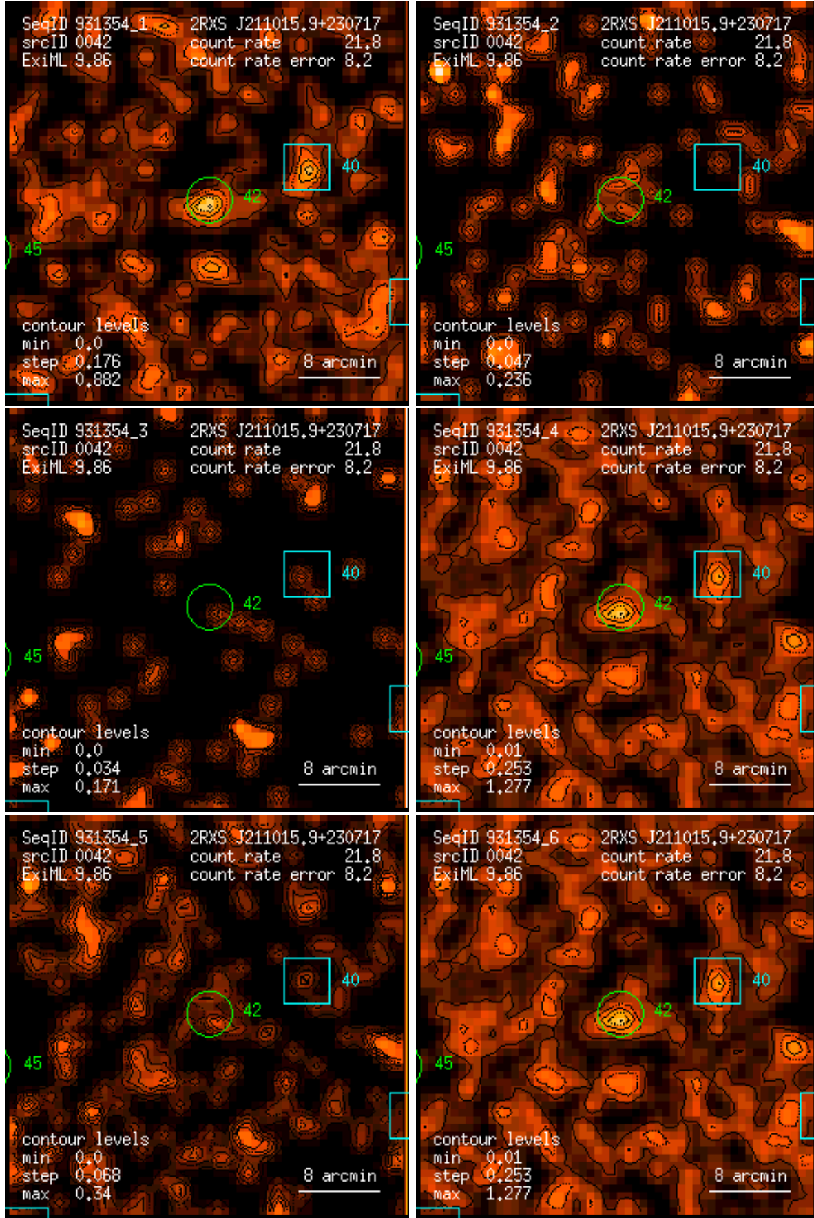
Figure 42: RASS 931354: detection 0042: band rate images, Gaussian filter: (1) PSPC channels 11 – 41, (2) 52 – 90, (3) 91 – 201, (4) 11 – 235, (5) 52 – 201, (6) 11 – 201. Broad band rates in counts/ks. Band rate contour levels in counts/ks/arcmin 2 .
