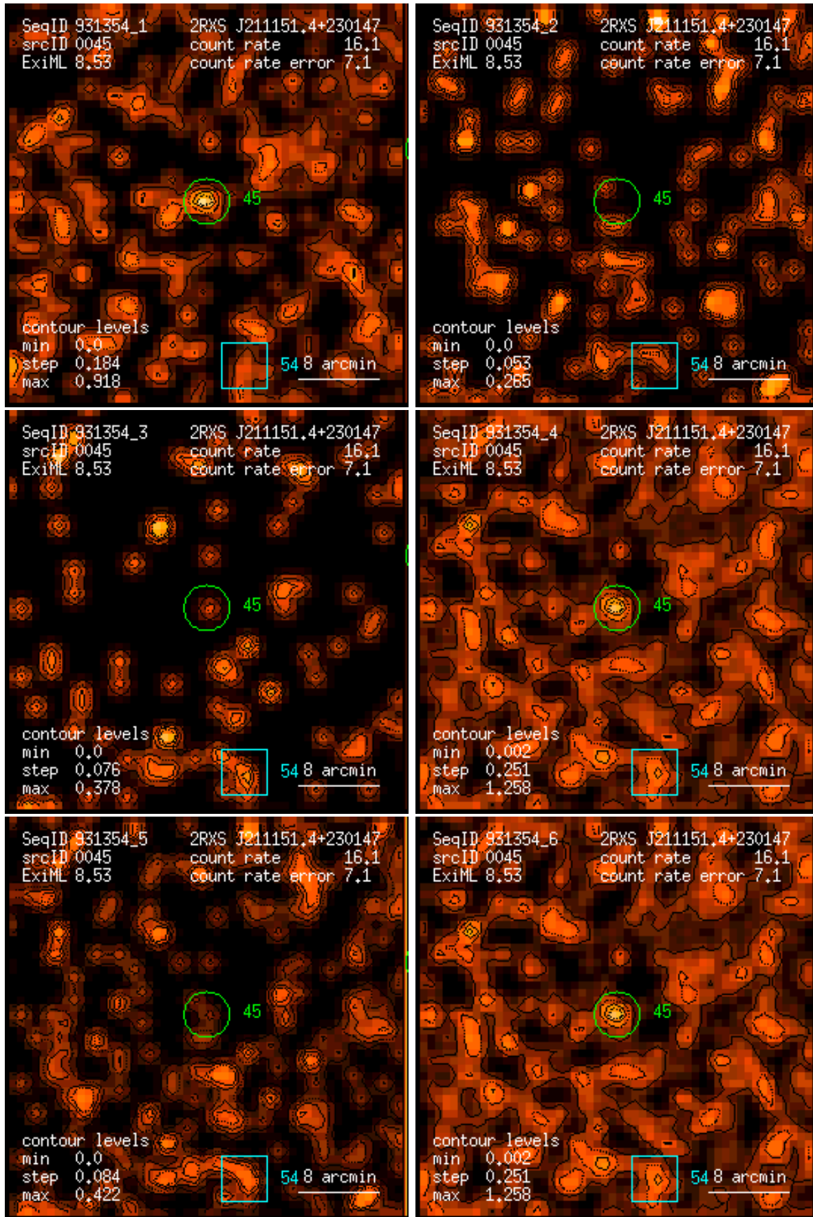
Figure 45: RASS 931354: detection 0045: band rate images, Gaussian filter: (1) PSPC channels 11 – 41, (2) 52 – 90, (3) 91 – 201, (4) 11 – 235, (5) 52 – 201, (6) 11 – 201. Broad band rates in counts/ks. Band rate contour levels in counts/ks/arcmin 2 .
