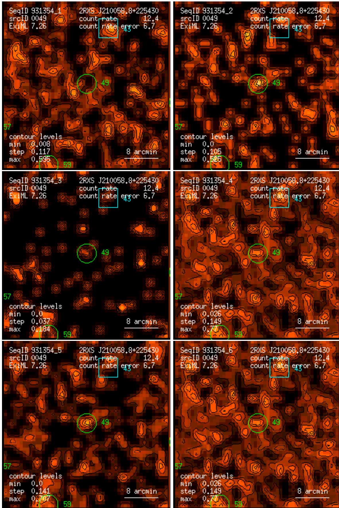
Figure 49: RASS 931354: detection 0049: band rate images, Gaussian filter: (1) PSPC channels 11 – 41, (2) 52 – 90, (3) 91 – 201, (4) 11 – 235, (5) 52 – 201, (6) 11 – 201. Broad band rates in counts/ks. Band rate contour levels in counts/ks/arcmin 2 .
