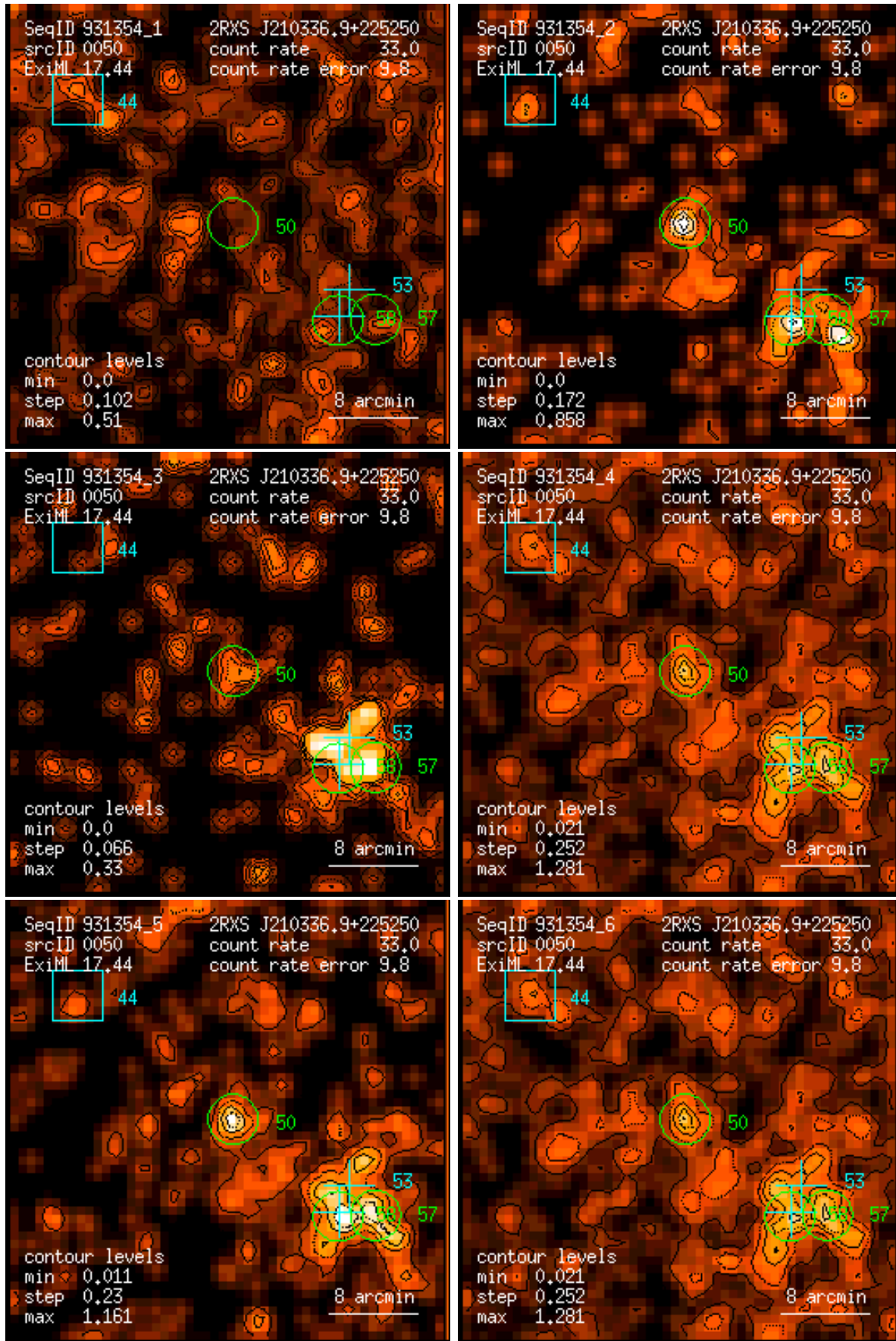
Figure 50: RASS 931354: detection 0050: band rate images, Gaussian filter: (1) PSPC channels 11 – 41, (2) 52 – 90, (3) 91 – 201, (4) 11 – 235, (5) 52 – 201, (6) 11 – 201. Broad band rates in counts/ks. Band rate contour levels in counts/ks/arcmin 2 .
