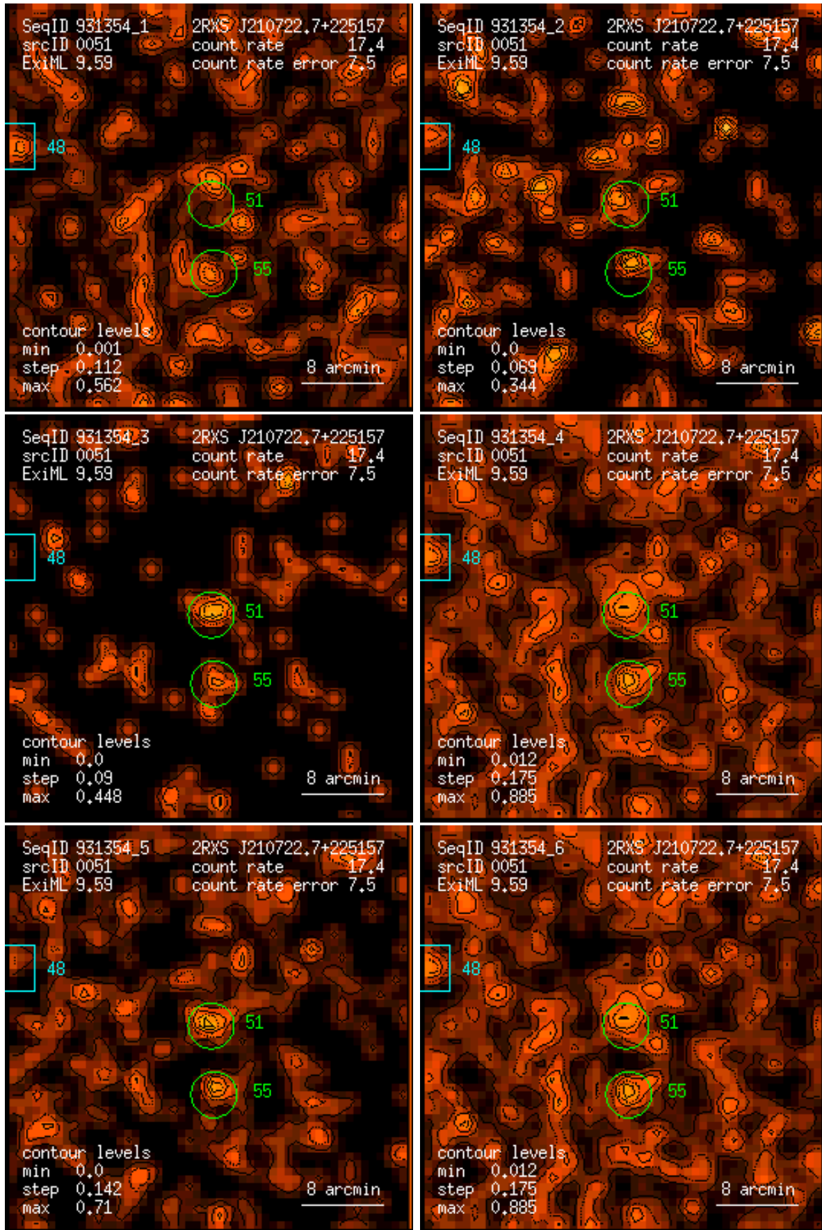
Figure 51: RASS 931354: detection 0051: band rate images, Gaussian filter: (1) PSPC channels 11 – 41, (2) 52 – 90, (3) 91 – 201, (4) 11 – 235, (5) 52 – 201, (6) 11 – 201. Broad band rates in counts/ks. Band rate contour levels in counts/ks/arcmin 2 .
