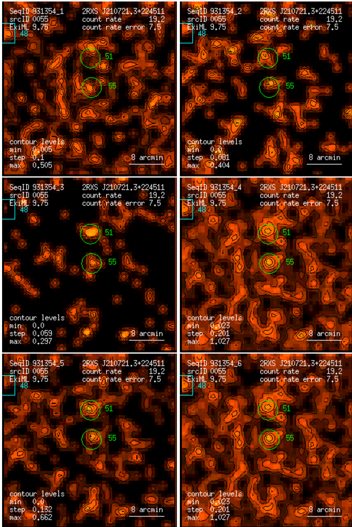
Figure 55: RASS 931354: detection 0055: band rate images, Gaussian filter: (1) PSPC channels 11 – 41, (2) 52 – 90, (3) 91 – 201, (4) 11 – 235, (5) 52 – 201, (6) 11 – 201. Broad band rates in counts/ks. Band rate contour levels in counts/ks/arcmin 2 .
