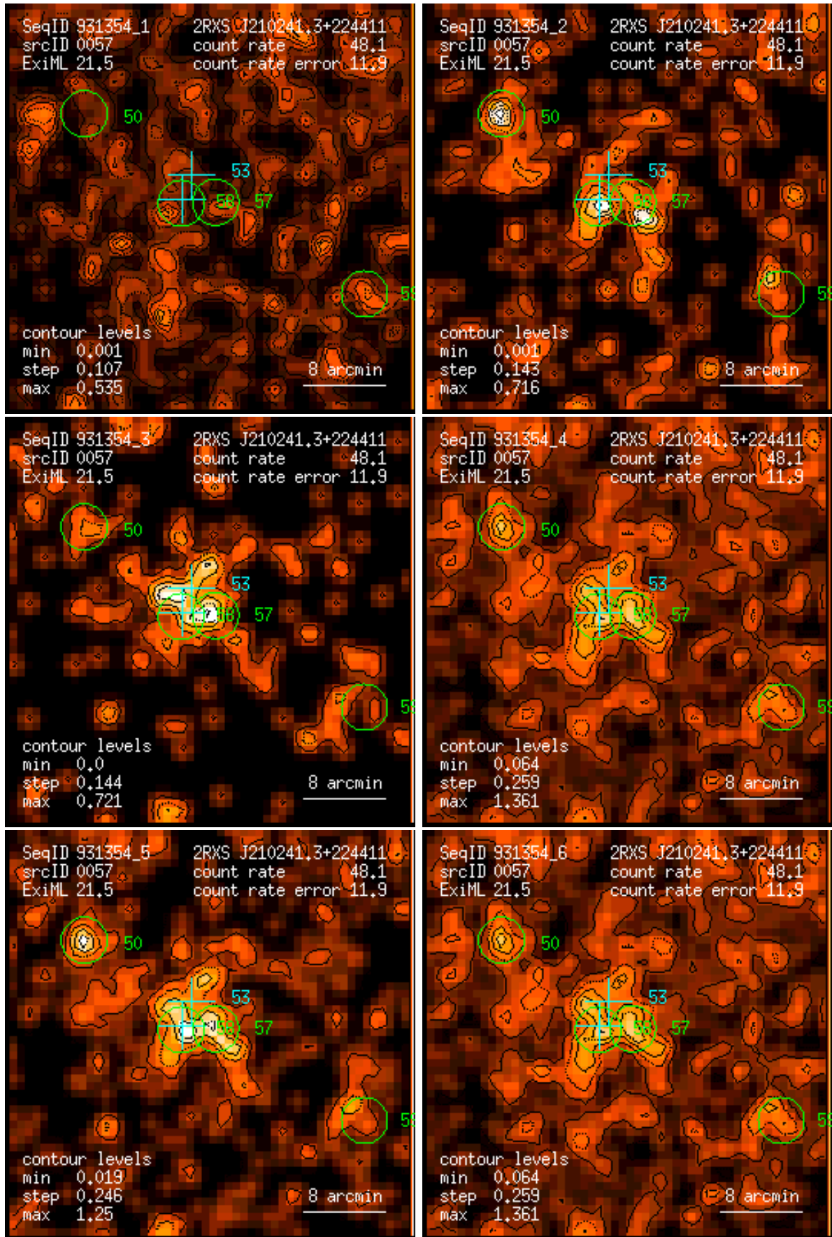
Figure 57: RASS 931354: detection 0057: band rate images, Gaussian filter: (1) PSPC channels 11 – 41, (2) 52 – 90, (3) 91 – 201, (4) 11 – 235, (5) 52 – 201, (6) 11 – 201. Broad band rates in counts/ks. Band rate contour levels in counts/ks/arcmin 2 .
