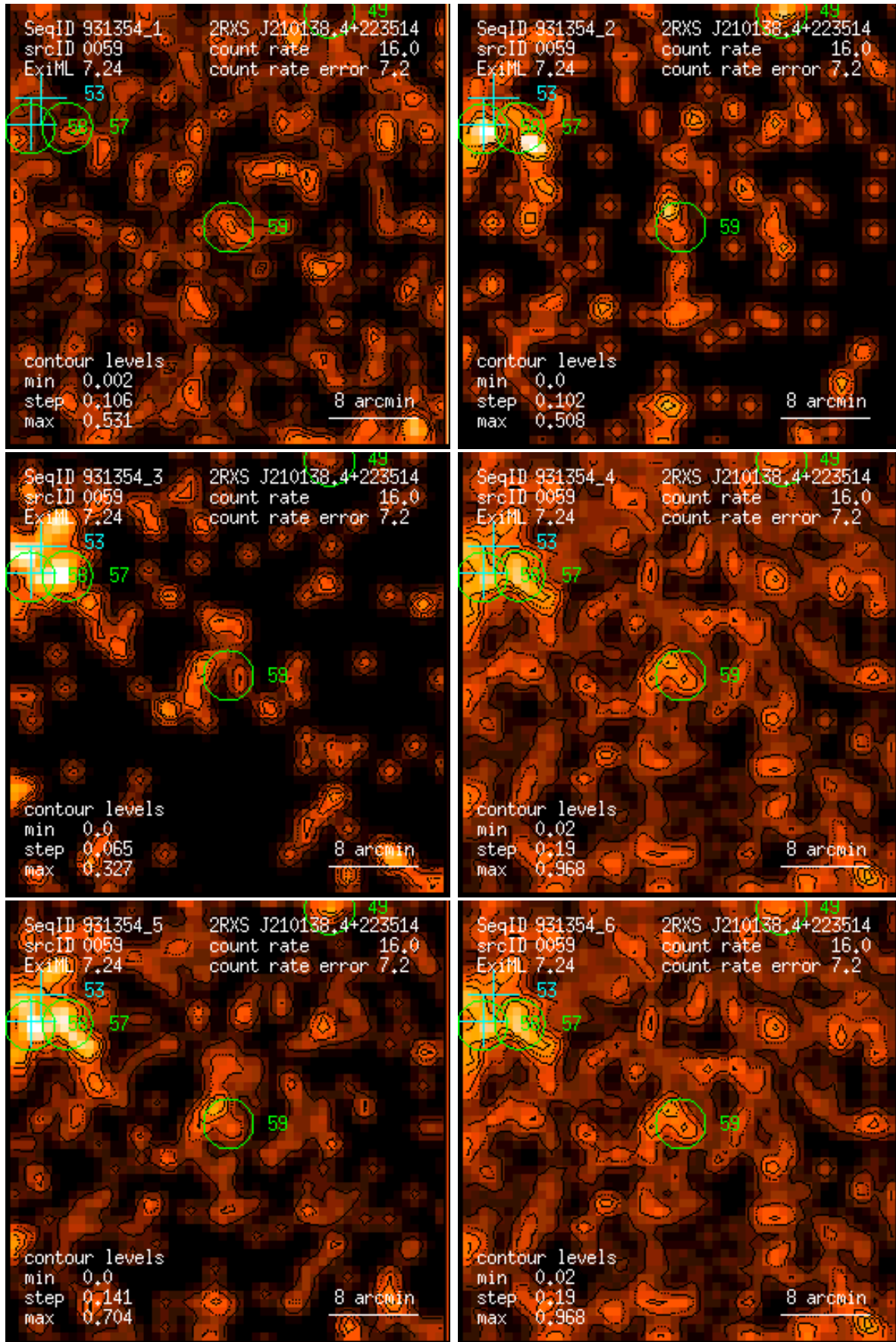
Figure 59: RASS 931354: detection 0059: band rate images, Gaussian filter: (1) PSPC channels 11 – 41, (2) 52 – 90, (3) 91 – 201, (4) 11 – 235, (5) 52 – 201, (6) 11 – 201. Broad band rates in counts/ks. Band rate contour levels in counts/ks/arcmin 2 .
