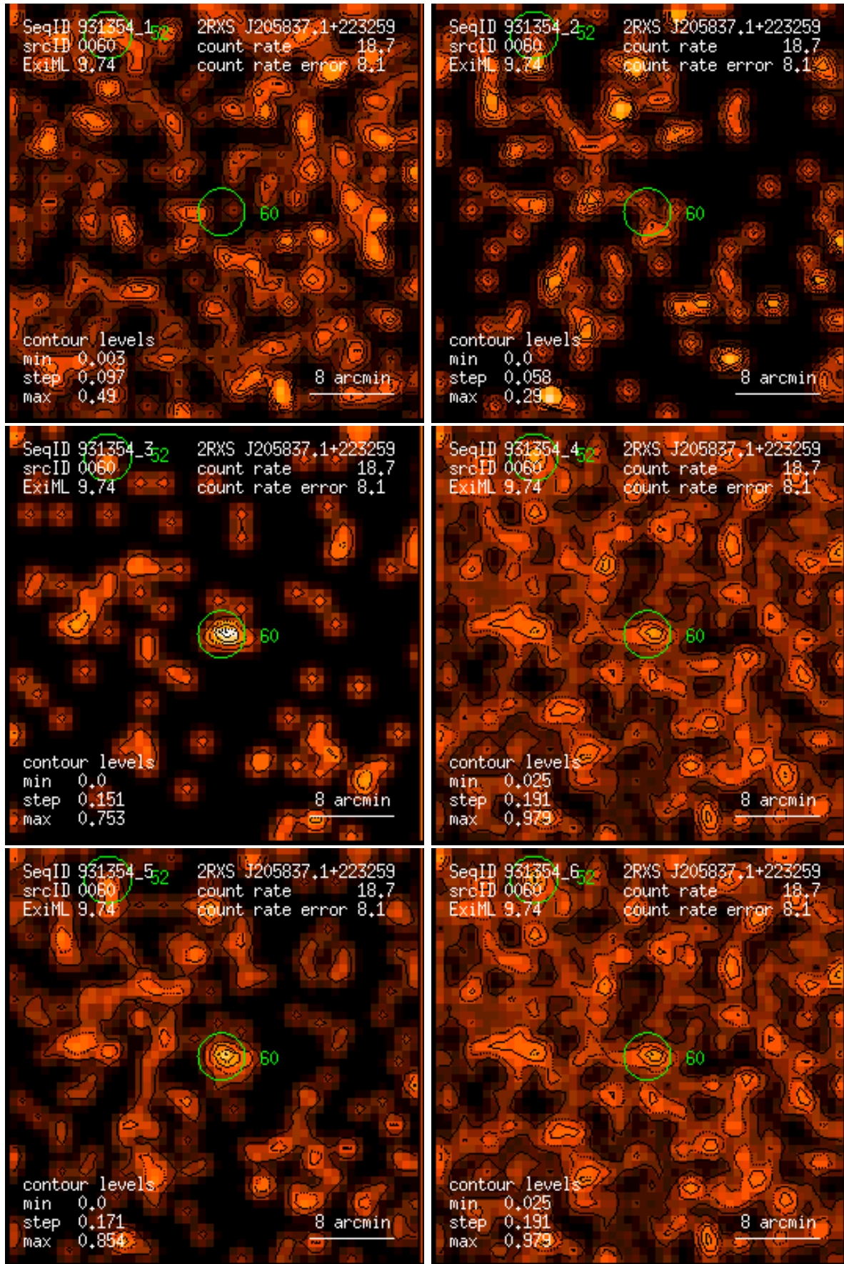
Figure 60: RASS 931354: detection 0060: band rate images, Gaussian filter: (1) PSPC channels 11 – 41, (2) 52 – 90, (3) 91 – 201, (4) 11 – 235, (5) 52 – 201, (6) 11 – 201. Broad band rates in counts/ks. Band rate contour levels in counts/ks/arcmin 2 .
