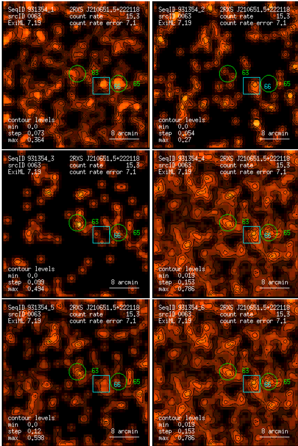
Figure 63: RASS 931354: detection 0063: band rate images, Gaussian filter: (1) PSPC channels 11 – 41, (2) 52 – 90, (3) 91 – 201, (4) 11 – 235, (5) 52 – 201, (6) 11 – 201. Broad band rates in counts/ks. Band rate contour levels in counts/ks/arcmin 2 .
