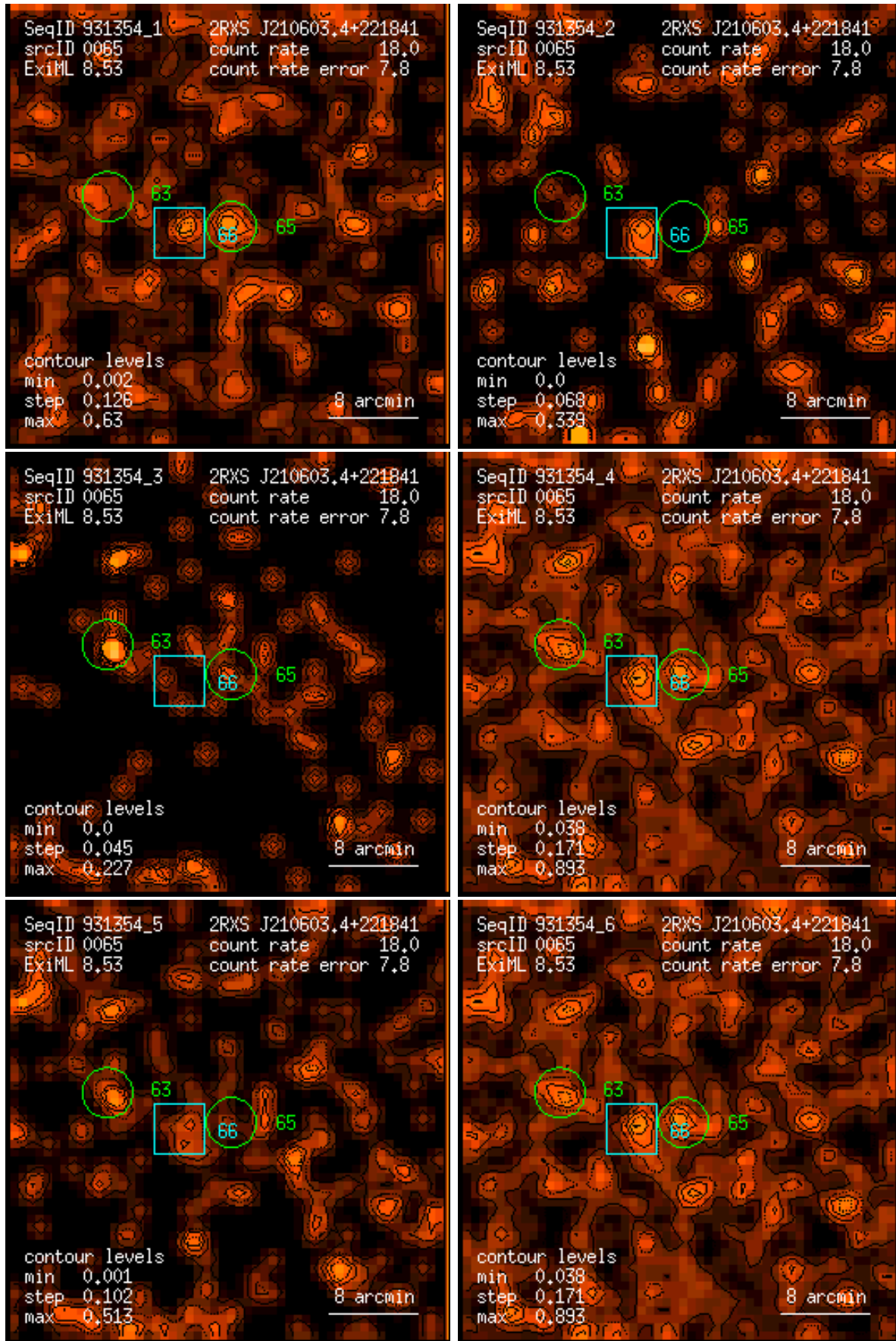
Figure 65: RASS 931354: detection 0065: band rate images, Gaussian filter: (1) PSPC channels 11 – 41, (2) 52 – 90, (3) 91 – 201, (4) 11 – 235, (5) 52 – 201, (6) 11 – 201. Broad band rates in counts/ks. Band rate contour levels in counts/ks/arcmin 2 .
