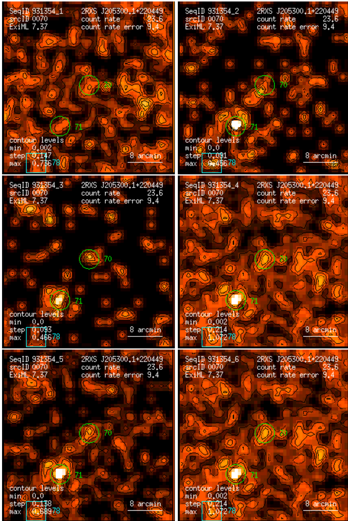
Figure 70: RASS 931354: detection 0070: band rate images, Gaussian filter: (1) PSPC channels 11 – 41, (2) 52 – 90, (3) 91 – 201, (4) 11 – 235, (5) 52 – 201, (6) 11 – 201. Broad band rates in counts/ks. Band rate contour levels in counts/ks/arcmin 2 .
