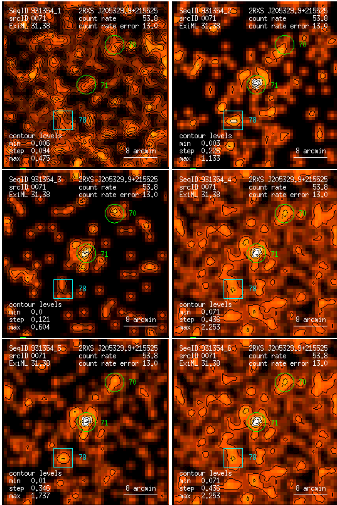
Figure 71: RASS 931354: detection 0071: band rate images, Gaussian filter: (1) PSPC channels 11 – 41, (2) 52 – 90, (3) 91 – 201, (4) 11 – 235, (5) 52 – 201, (6) 11 – 201. Broad band rates in counts/ks. Band rate contour levels in counts/ks/arcmin 2 .
