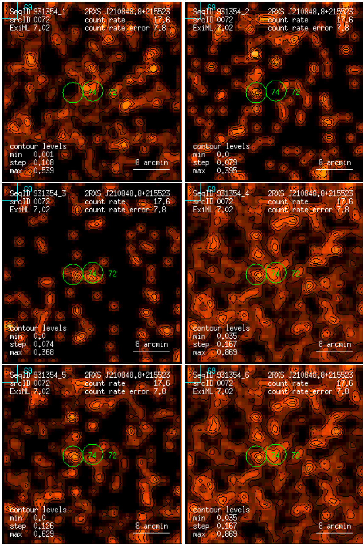
Figure 72: RASS 931354: detection 0072: band rate images, Gaussian filter: (1) PSPC channels 11 – 41, (2) 52 – 90, (3) 91 – 201, (4) 11 – 235, (5) 52 – 201, (6) 11 – 201. Broad band rates in counts/ks. Band rate contour levels in counts/ks/arcmin 2 .
