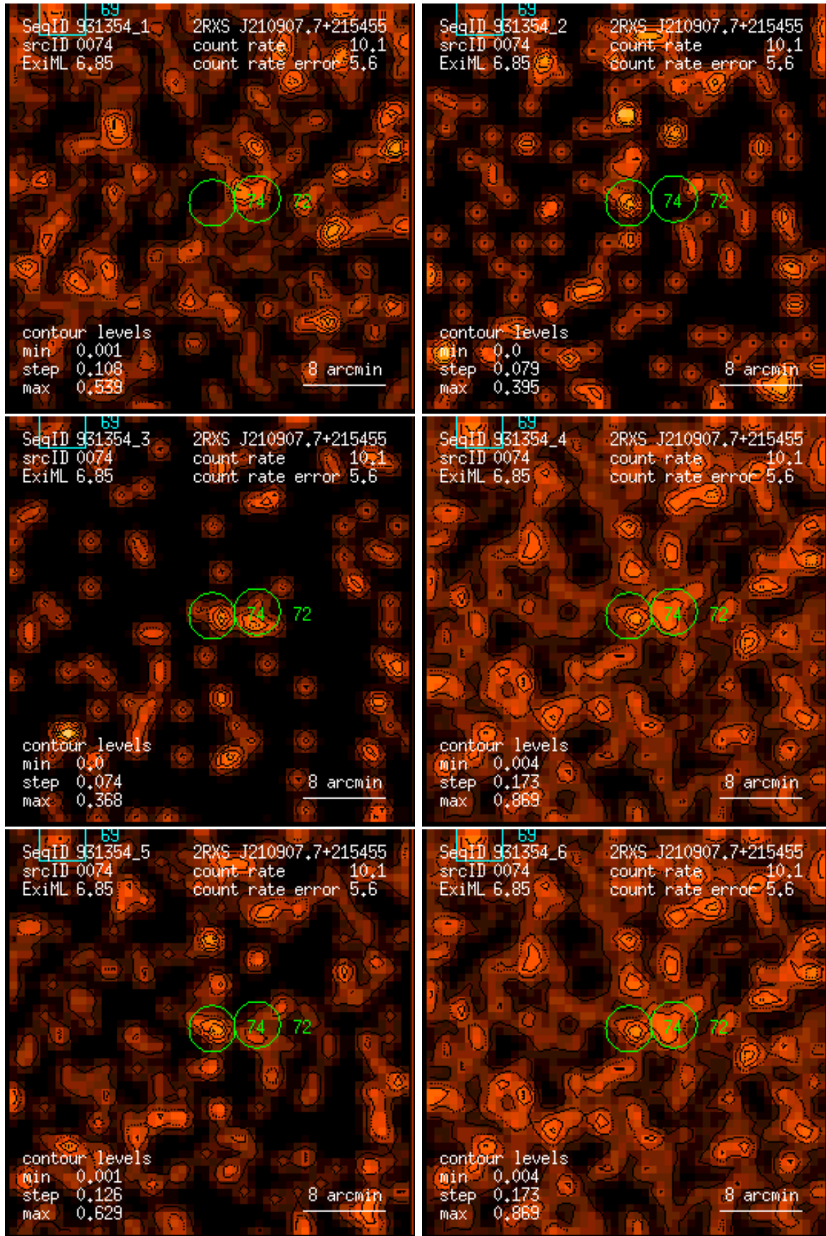
Figure 74: RASS 931354: detection 0074: band rate images, Gaussian filter: (1) PSPC channels 11 – 41, (2) 52 – 90, (3) 91 – 201, (4) 11 – 235, (5) 52 – 201, (6) 11 – 201. Broad band rates in counts/ks. Band rate contour levels in counts/ks/arcmin 2 .
