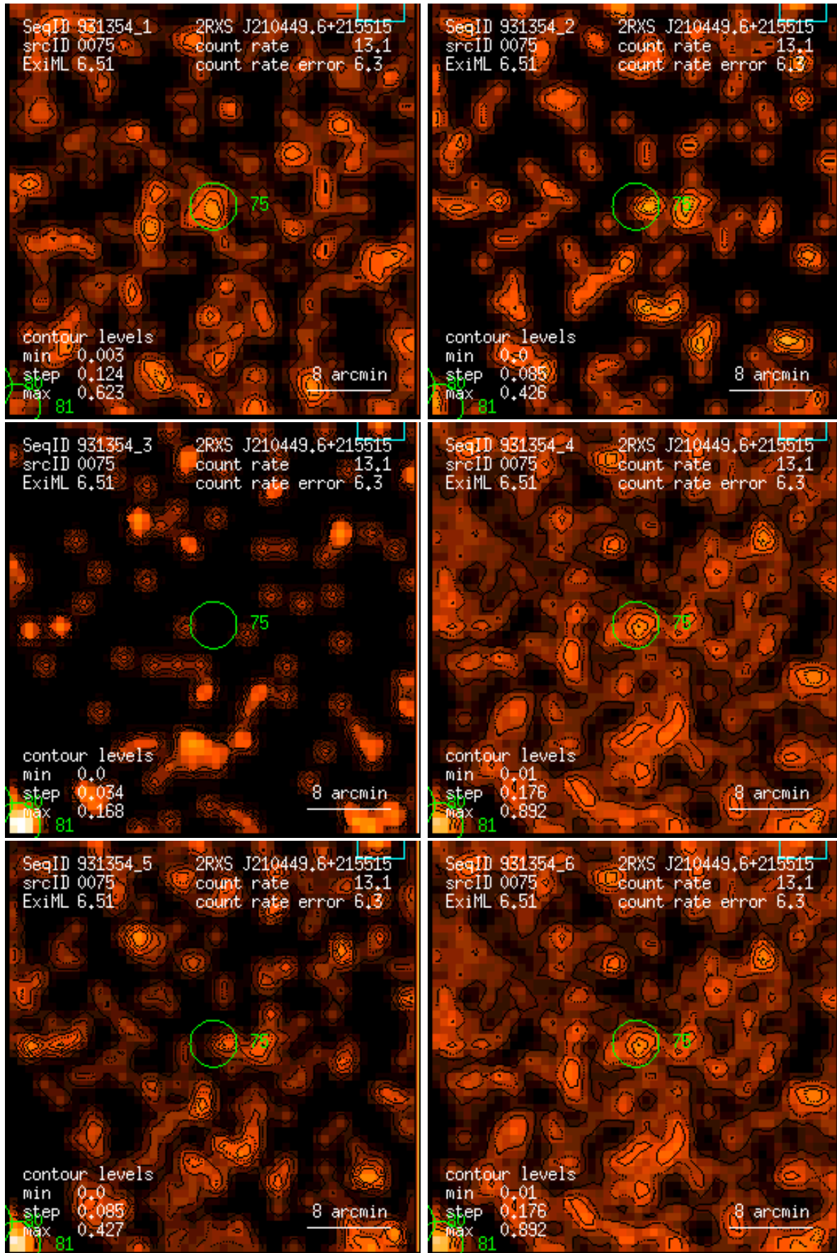
Figure 75: RASS 931354: detection 0075: band rate images, Gaussian filter: (1) PSPC channels 11 – 41, (2) 52 – 90, (3) 91 – 201, (4) 11 – 235, (5) 52 – 201, (6) 11 – 201. Broad band rates in counts/ks. Band rate contour levels in counts/ks/arcmin 2 .
