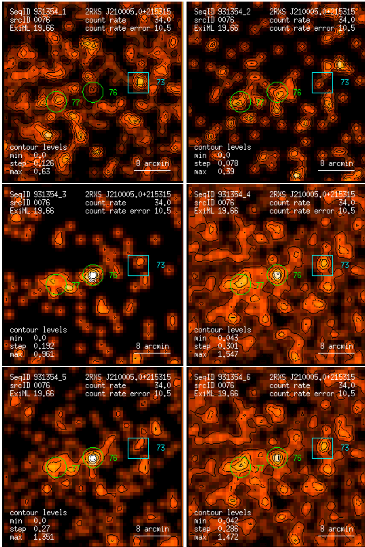
Figure 76: RASS 931354: detection 0076: band rate images, Gaussian filter: (1) PSPC channels 11 – 41, (2) 52 – 90, (3) 91 – 201, (4) 11 – 235, (5) 52 – 201, (6) 11 – 201. Broad band rates in counts/ks. Band rate contour levels in counts/ks/arcmin 2 .
