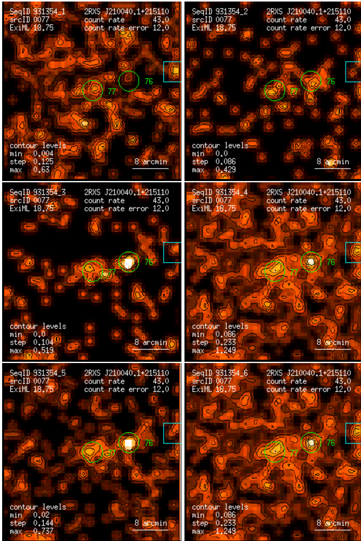
Figure 77: RASS 931354: detection 0077: band rate images, Gaussian filter: (1) PSPC channels 11 – 41, (2) 52 – 90, (3) 91 – 201, (4) 11 – 235, (5) 52 – 201, (6) 11 – 201. Broad band rates in counts/ks. Band rate contour levels in counts/ks/arcmin 2 .
