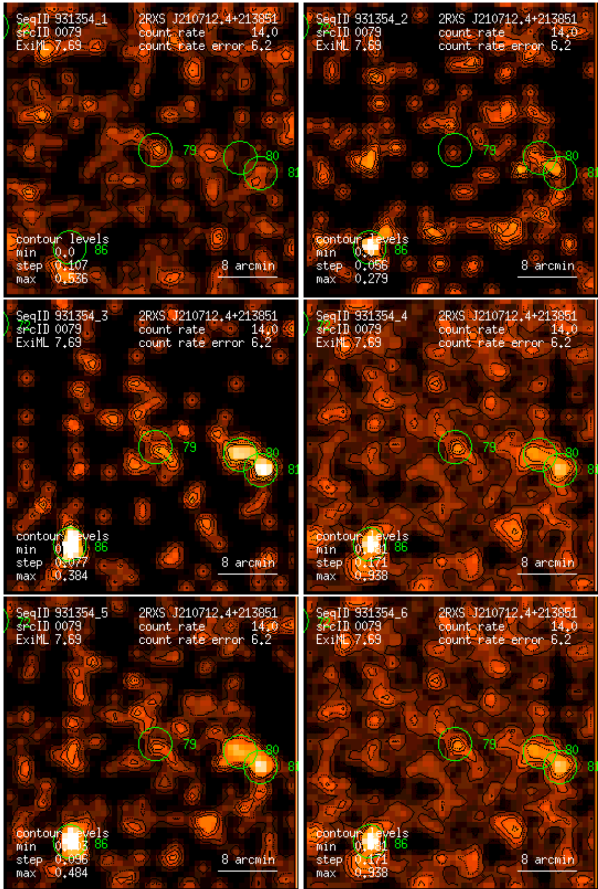
Figure 79: RASS 931354: detection 0079: band rate images, Gaussian filter: (1) PSPC channels 11 – 41, (2) 52 – 90, (3) 91 – 201, (4) 11 – 235, (5) 52 – 201, (6) 11 – 201. Broad band rates in counts/ks. Band rate contour levels in counts/ks/arcmin 2 .
