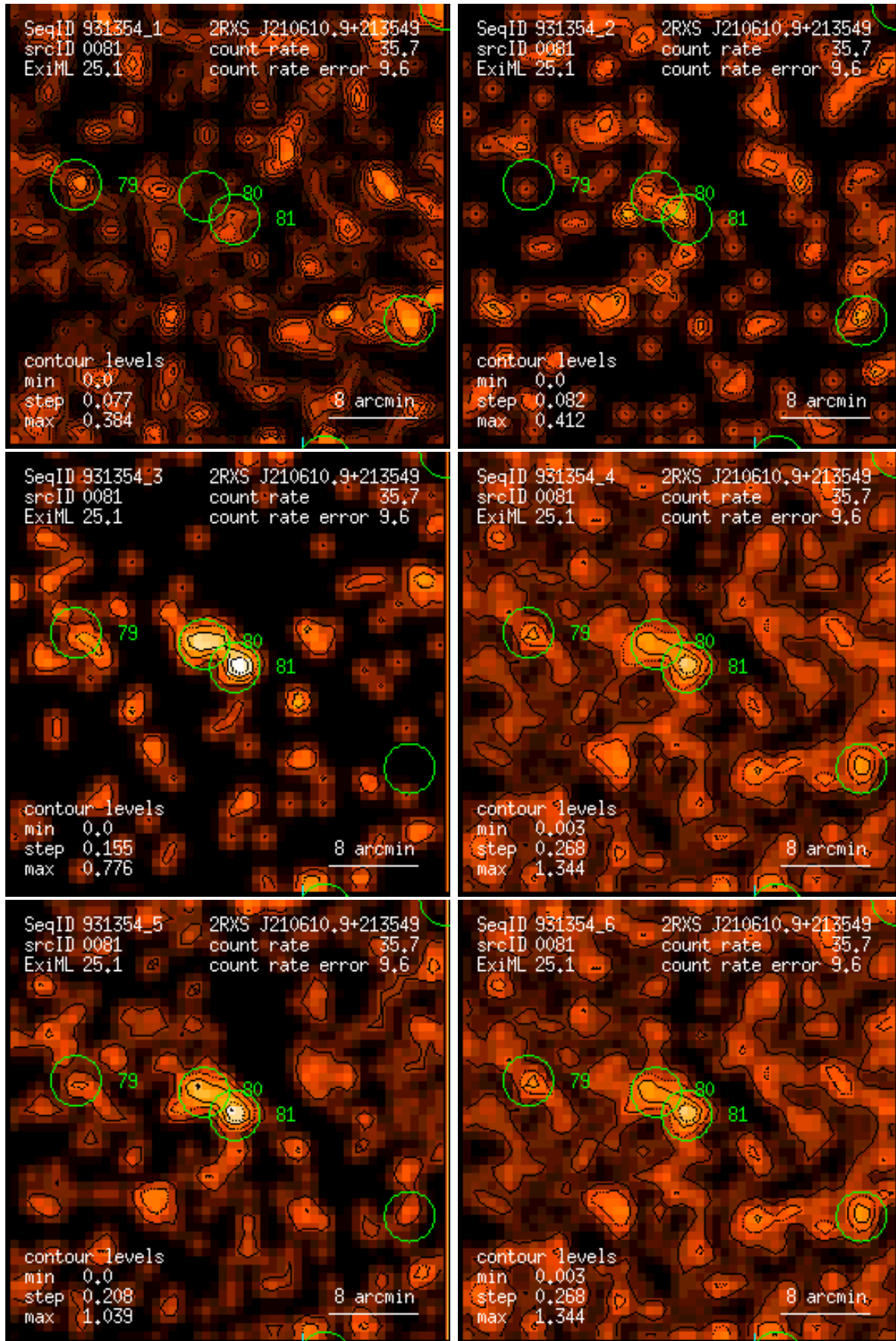
Figure 81: RASS 931354: detection 0081: band rate images, Gaussian filter: (1) PSPC channels 11 – 41, (2) 52 – 90, (3) 91 – 201, (4) 11 – 235, (5) 52 – 201, (6) 11 – 201. Broad band rates in counts/ks. Band rate contour levels in counts/ks/arcmin 2 .
