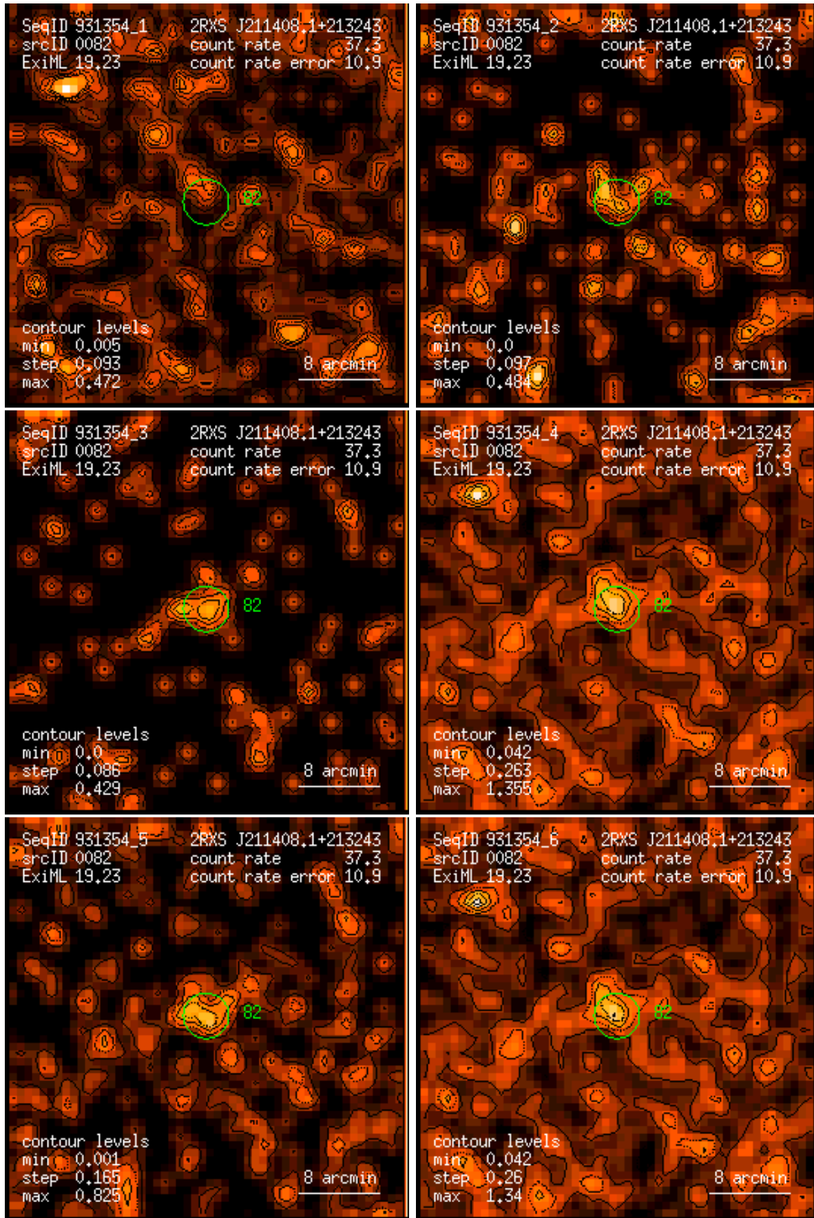
Figure 82: RASS 931354: detection 0082: band rate images, Gaussian filter: (1) PSPC channels 11 – 41, (2) 52 – 90, (3) 91 – 201, (4) 11 – 235, (5) 52 – 201, (6) 11 – 201. Broad band rates in counts/ks. Band rate contour levels in counts/ks/arcmin 2 .
