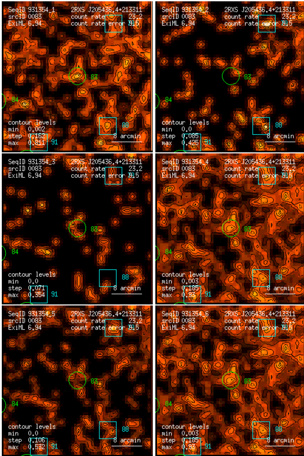
Figure 83: RASS 931354: detection 0083: band rate images, Gaussian filter: (1) PSPC channels 11 – 41, (2) 52 – 90, (3) 91 – 201, (4) 11 – 235, (5) 52 – 201, (6) 11 – 201. Broad band rates in counts/ks. Band rate contour levels in counts/ks/arcmin 2 .
