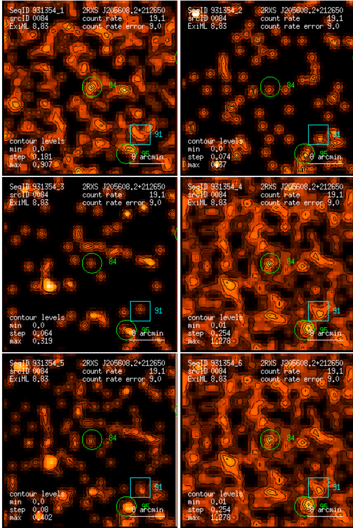
Figure 84: RASS 931354: detection 0084: band rate images, Gaussian filter: (1) PSPC channels 11 – 41, (2) 52 – 90, (3) 91 – 201, (4) 11 – 235, (5) 52 – 201, (6) 11 – 201. Broad band rates in counts/ks. Band rate contour levels in counts/ks/arcmin 2 .
