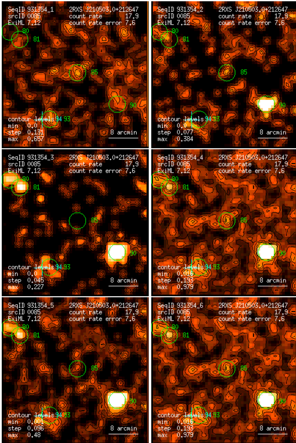
Figure 85: RASS 931354: detection 0085: band rate images, Gaussian filter: (1) PSPC channels 11 – 41, (2) 52 – 90, (3) 91 – 201, (4) 11 – 235, (5) 52 – 201, (6) 11 – 201. Broad band rates in counts/ks. Band rate contour levels in counts/ks/arcmin 2 .
