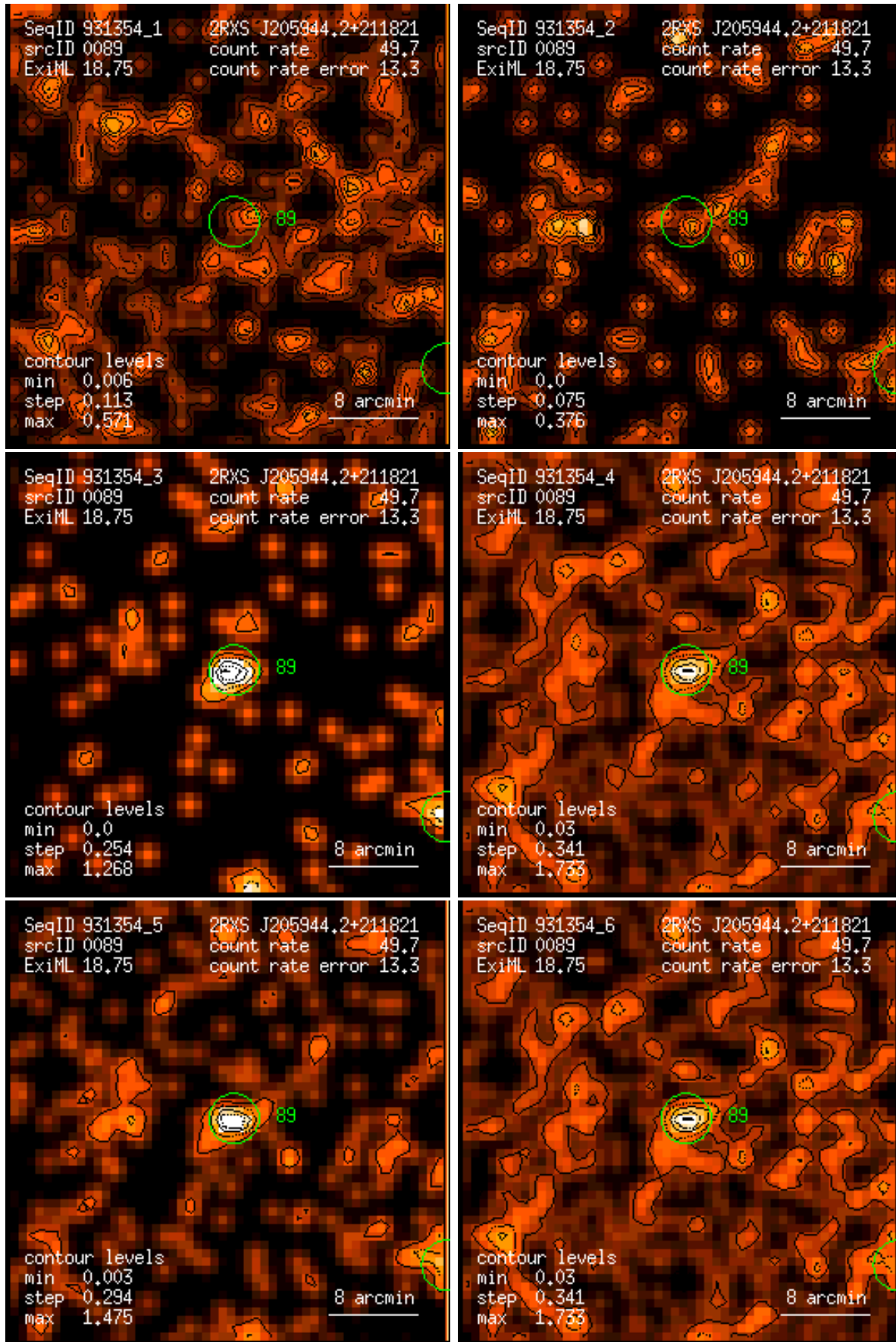
Figure 89: RASS 931354: detection 0089: band rate images, Gaussian filter: (1) PSPC channels 11 – 41, (2) 52 – 90, (3) 91 – 201, (4) 11 – 235, (5) 52 – 201, (6) 11 – 201. Broad band rates in counts/ks. Band rate contour levels in counts/ks/arcmin 2 .
