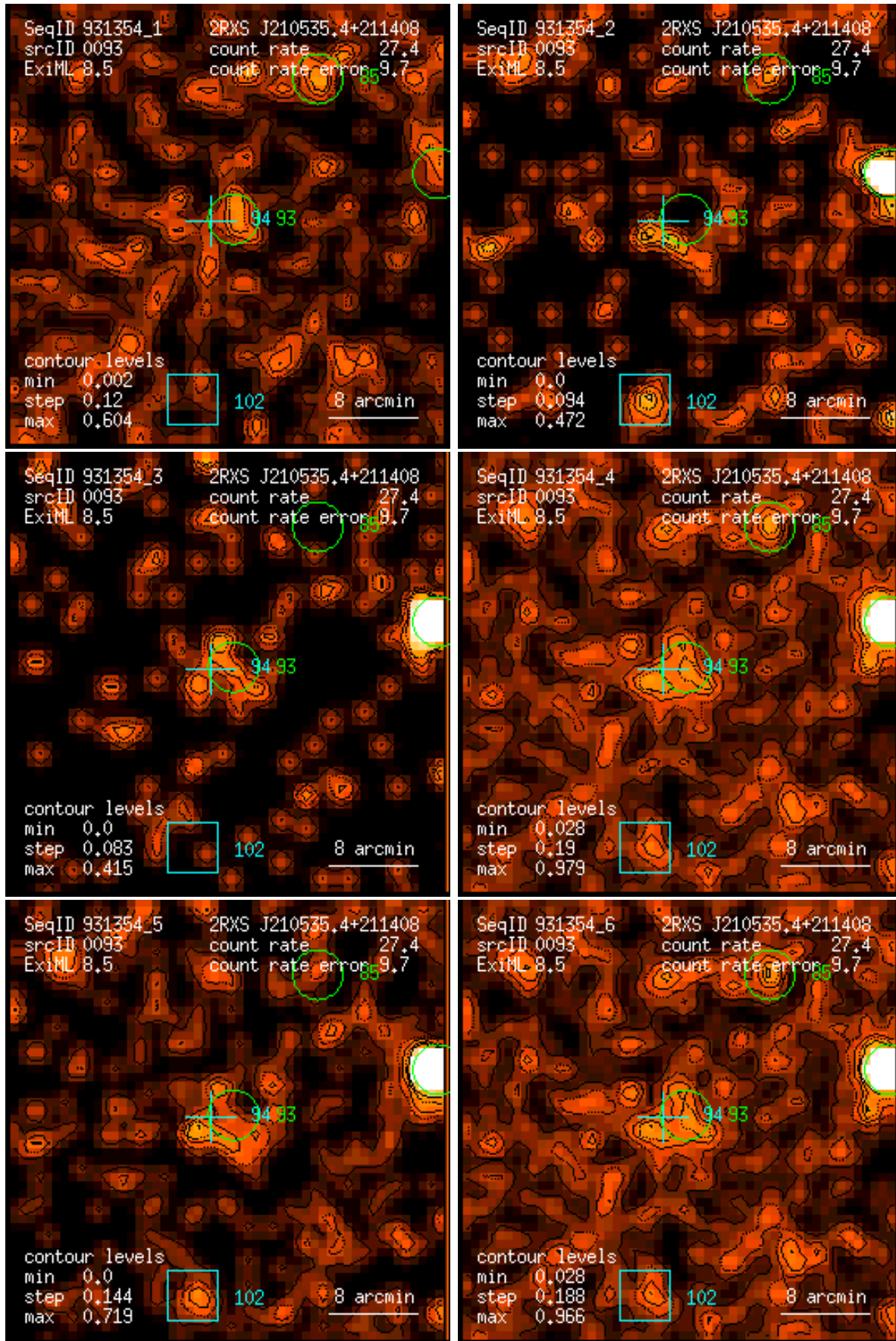
Figure 93: RASS 931354: detection 0093: band rate images, Gaussian filter: (1) PSPC channels 11 – 41, (2) 52 – 90, (3) 91 – 201, (4) 11 – 235, (5) 52 – 201, (6) 11 – 201. Broad band rates in counts/ks. Band rate contour levels in counts/ks/arcmin 2 .
