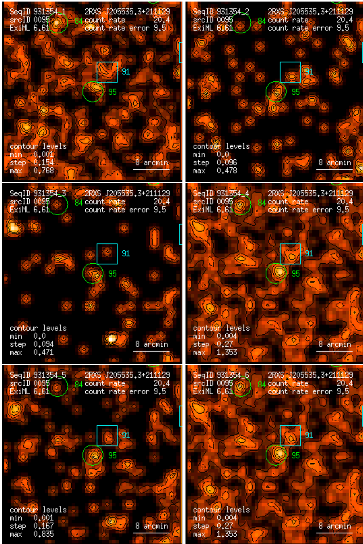
Figure 95: RASS 931354: detection 0095: band rate images, Gaussian filter: (1) PSPC channels 11 – 41, (2) 52 – 90, (3) 91 – 201, (4) 11 – 235, (5) 52 – 201, (6) 11 – 201. Broad band rates in counts/ks. Band rate contour levels in counts/ks/arcmin 2 .
