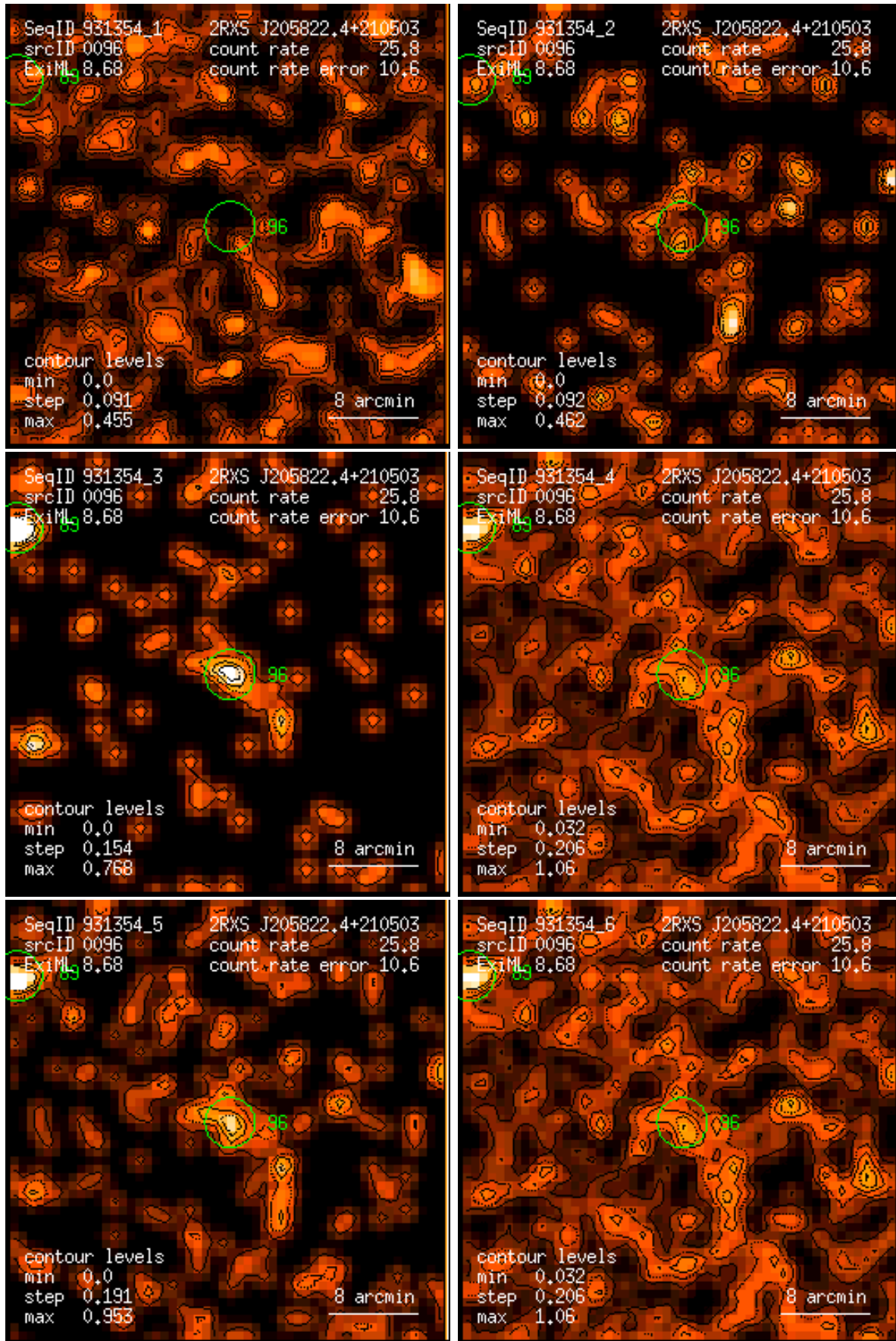
Figure 96: RASS 931354: detection 0096: band rate images, Gaussian filter: (1) PSPC channels 11 – 41, (2) 52 – 90, (3) 91 – 201, (4) 11 – 235, (5) 52 – 201, (6) 11 – 201. Broad band rates in counts/ks. Band rate contour levels in counts/ks/arcmin 2 .
