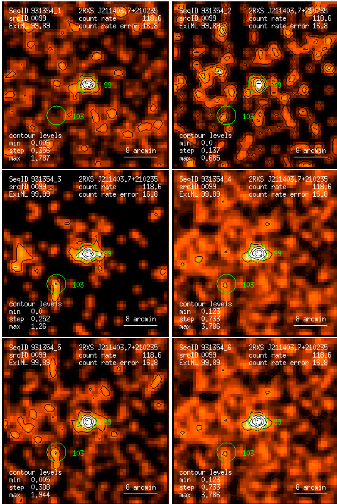
Figure 99: RASS 931354: detection 0099: band rate images, Gaussian filter: (1) PSPC channels 11 – 41, (2) 52 – 90, (3) 91 – 201, (4) 11 – 235, (5) 52 – 201, (6) 11 – 201. Broad band rates in counts/ks. Band rate contour levels in counts/ks/arcmin 2 .
