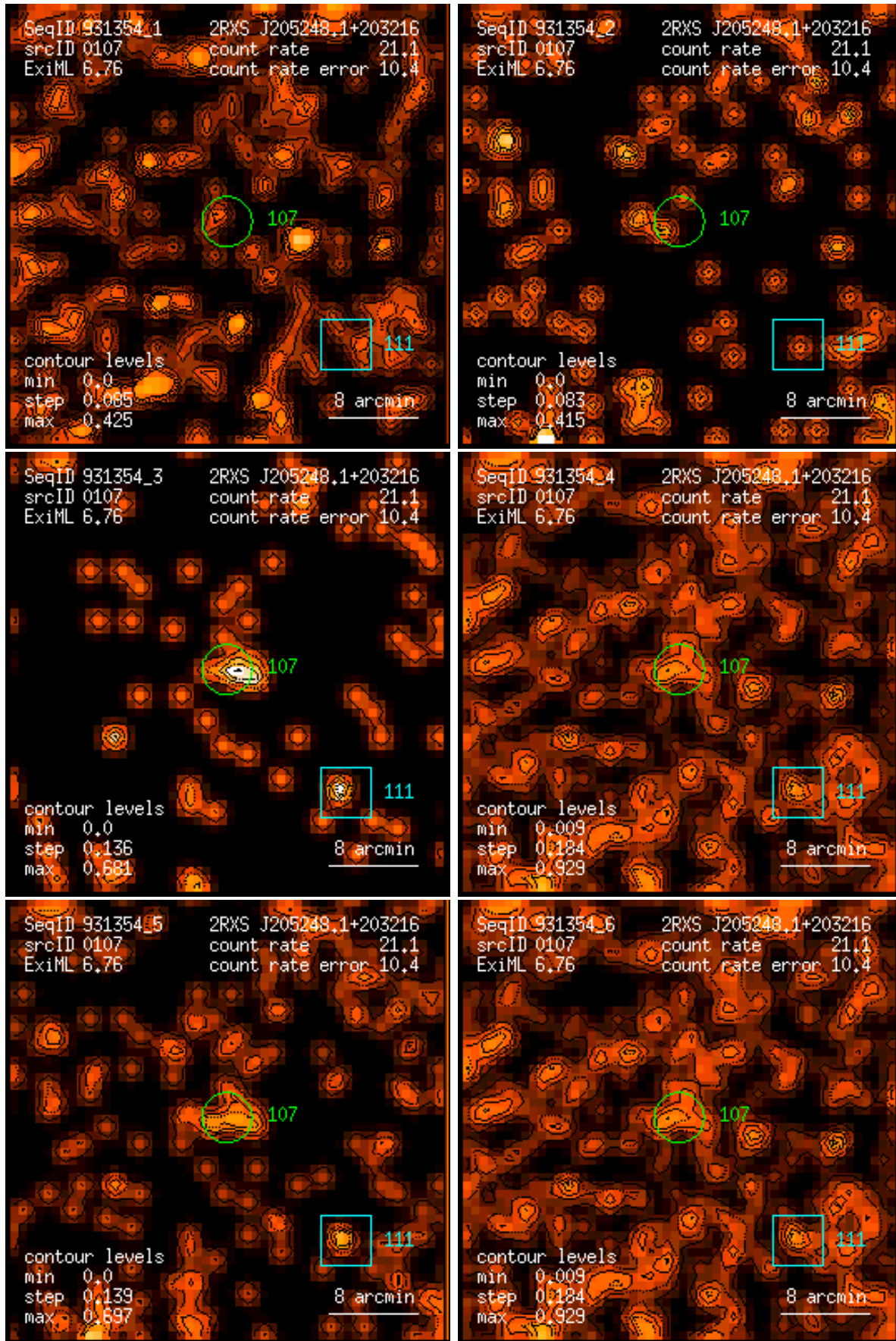
Figure 107: RASS 931354: detection 0107: band rate images, Gaussian filter: (1) PSPC channels 11 – 41, (2) 52 – 90, (3) 91 – 201, (4) 11 – 235, (5) 52 – 201, (6) 11 – 201. Broad band rates in counts/ks. Band rate contour levels in counts/ks/arcmin 2 .
