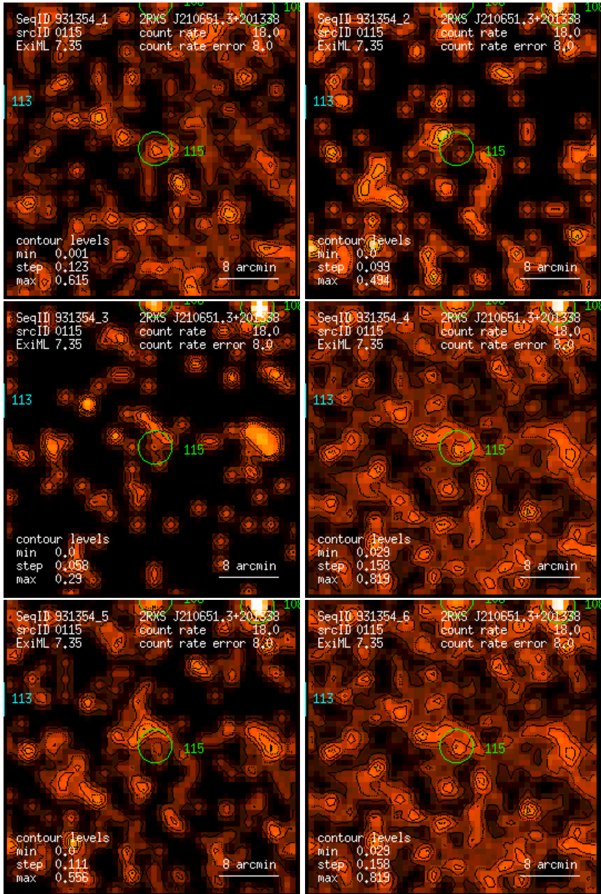
Figure 115: RASS 931354: detection 0115: band rate images, Gaussian filter: (1) PSPC channels 11 – 41, (2) 52 – 90, (3) 91 – 201, (4) 11 – 235, (5) 52 – 201, (6) 11 – 201. Broad band rates in counts/ks. Band rate contour levels in counts/ks/arcmin 2 .
