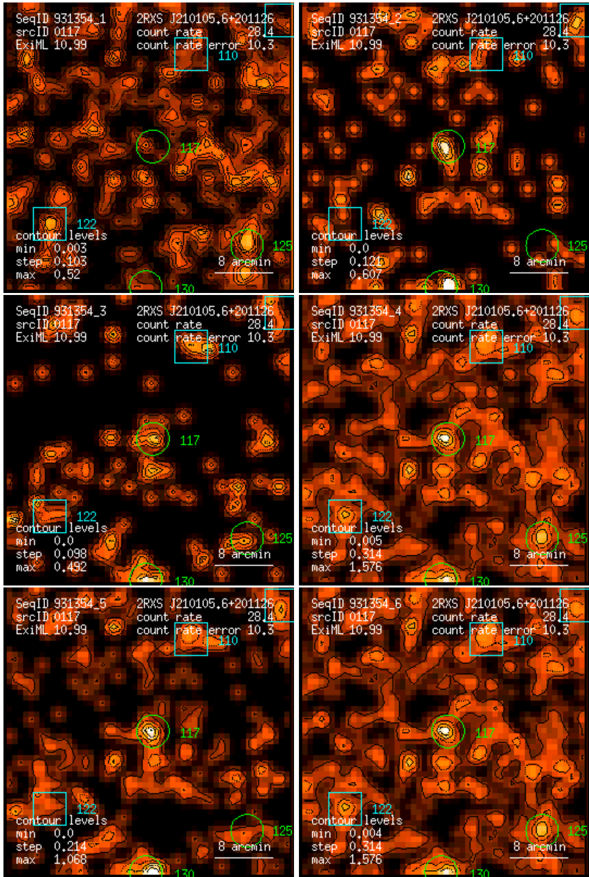
Figure 117: RASS 931354: detection 0117: band rate images, Gaussian filter: (1) PSPC channels 11 – 41, (2) 52 – 90, (3) 91 – 201, (4) 11 – 235, (5) 52 – 201, (6) 11 – 201. Broad band rates in counts/ks. Band rate contour levels in counts/ks/arcmin 2 .
