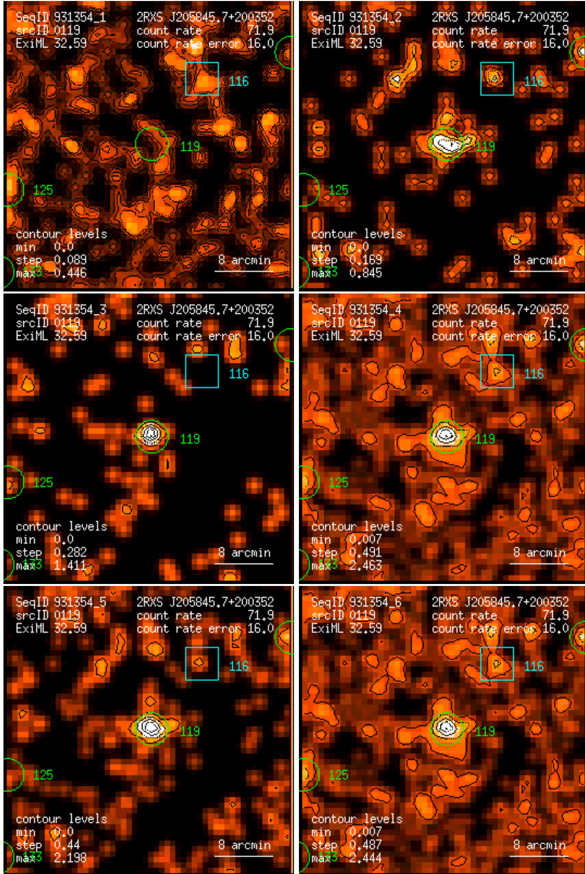
Figure 119: RASS 931354: detection 0119: band rate images, Gaussian filter: (1) PSPC channels 11 – 41, (2) 52 – 90, (3) 91 – 201, (4) 11 – 235, (5) 52 – 201, (6) 11 – 201. Broad band rates in counts/ks. Band rate contour levels in counts/ks/arcmin 2 .
