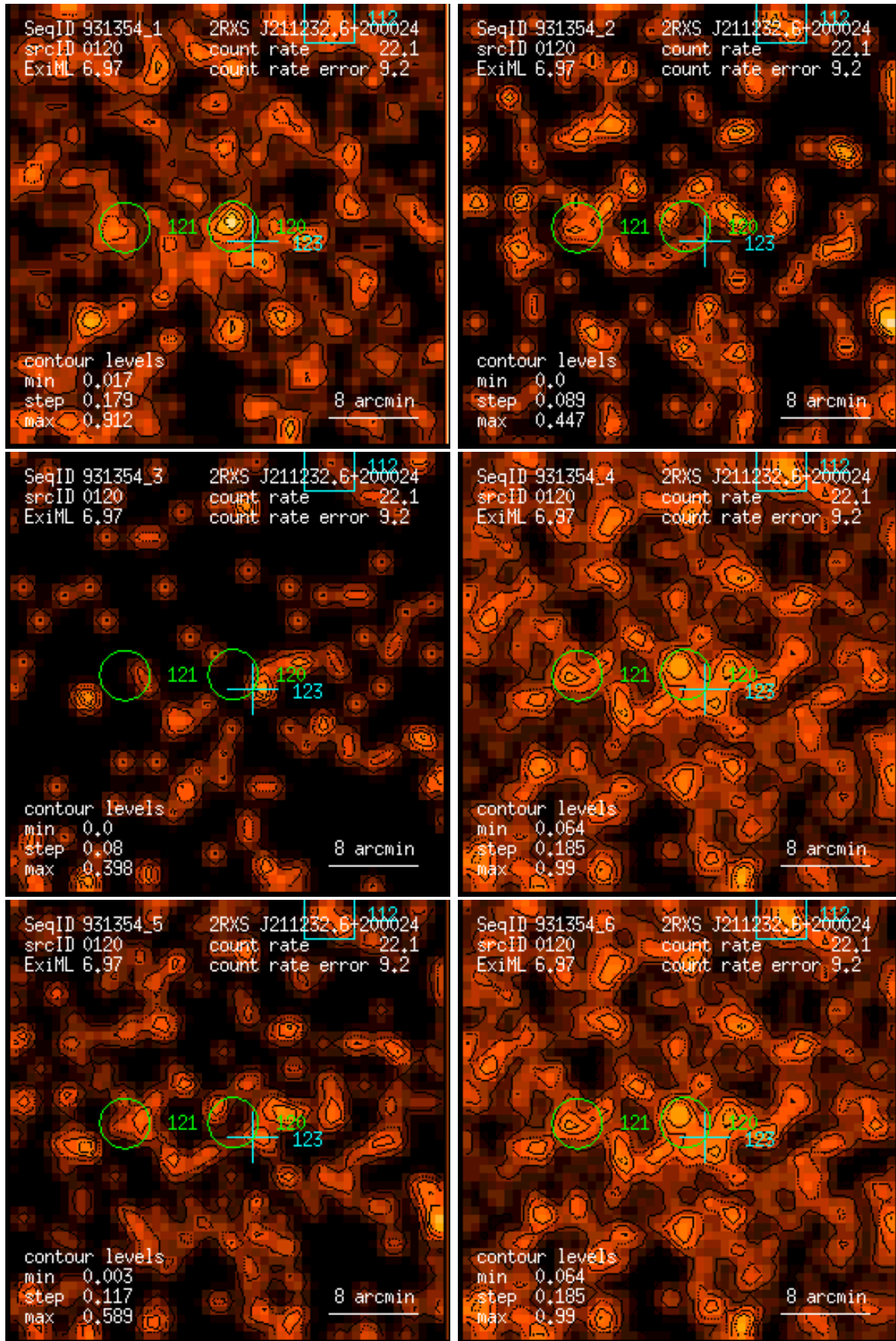
Figure 120: RASS 931354: detection 0120: band rate images, Gaussian filter: (1) PSPC channels 11 – 41, (2) 52 – 90, (3) 91 – 201, (4) 11 – 235, (5) 52 – 201, (6) 11 – 201. Broad band rates in counts/ks. Band rate contour levels in counts/ks/arcmin 2 .
