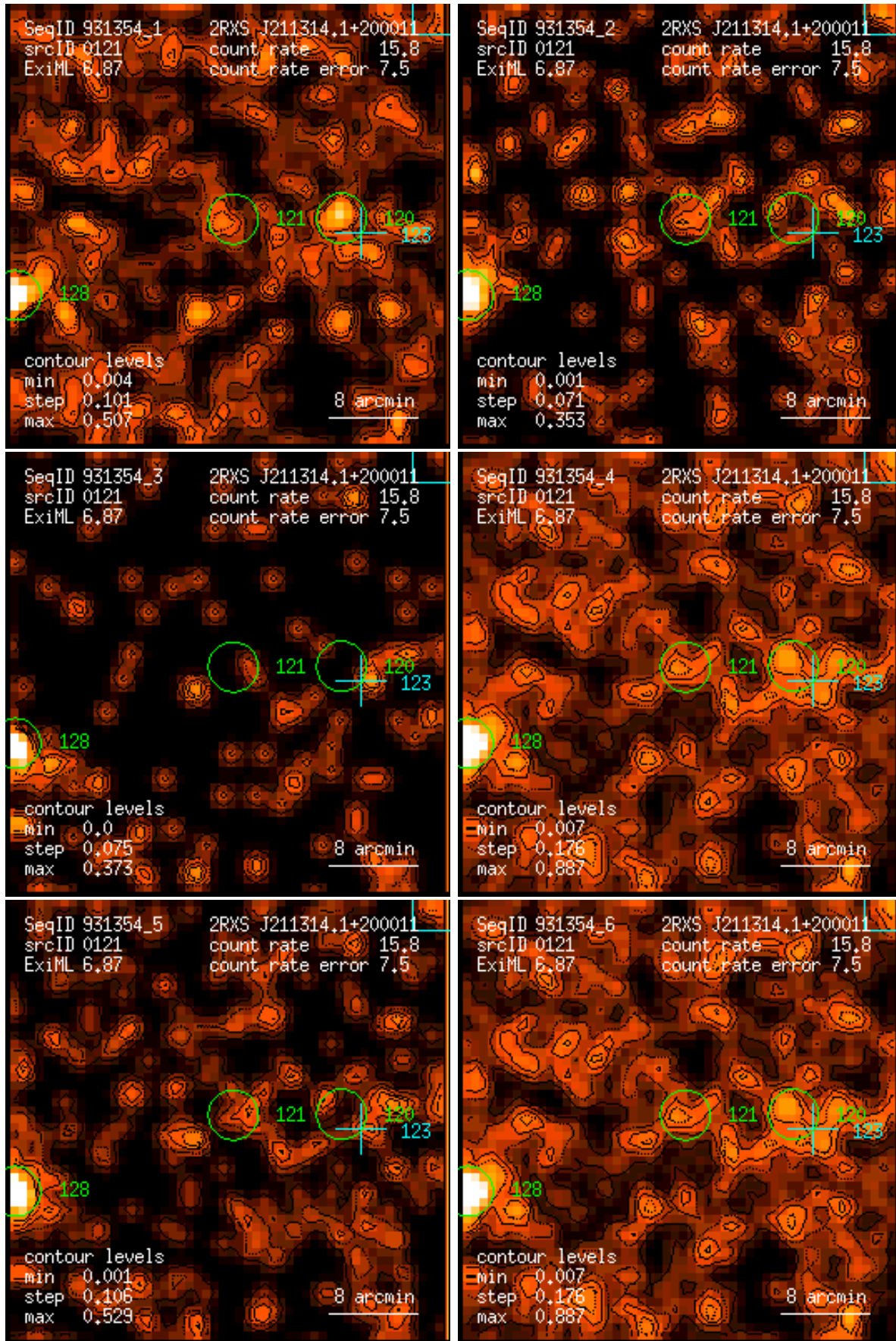
Figure 121: RASS 931354: detection 0121: band rate images, Gaussian filter: (1) PSPC channels 11 – 41, (2) 52 – 90, (3) 91 – 201, (4) 11 – 235, (5) 52 – 201, (6) 11 – 201. Broad band rates in counts/ks. Band rate contour levels in counts/ks/arcmin 2 .
