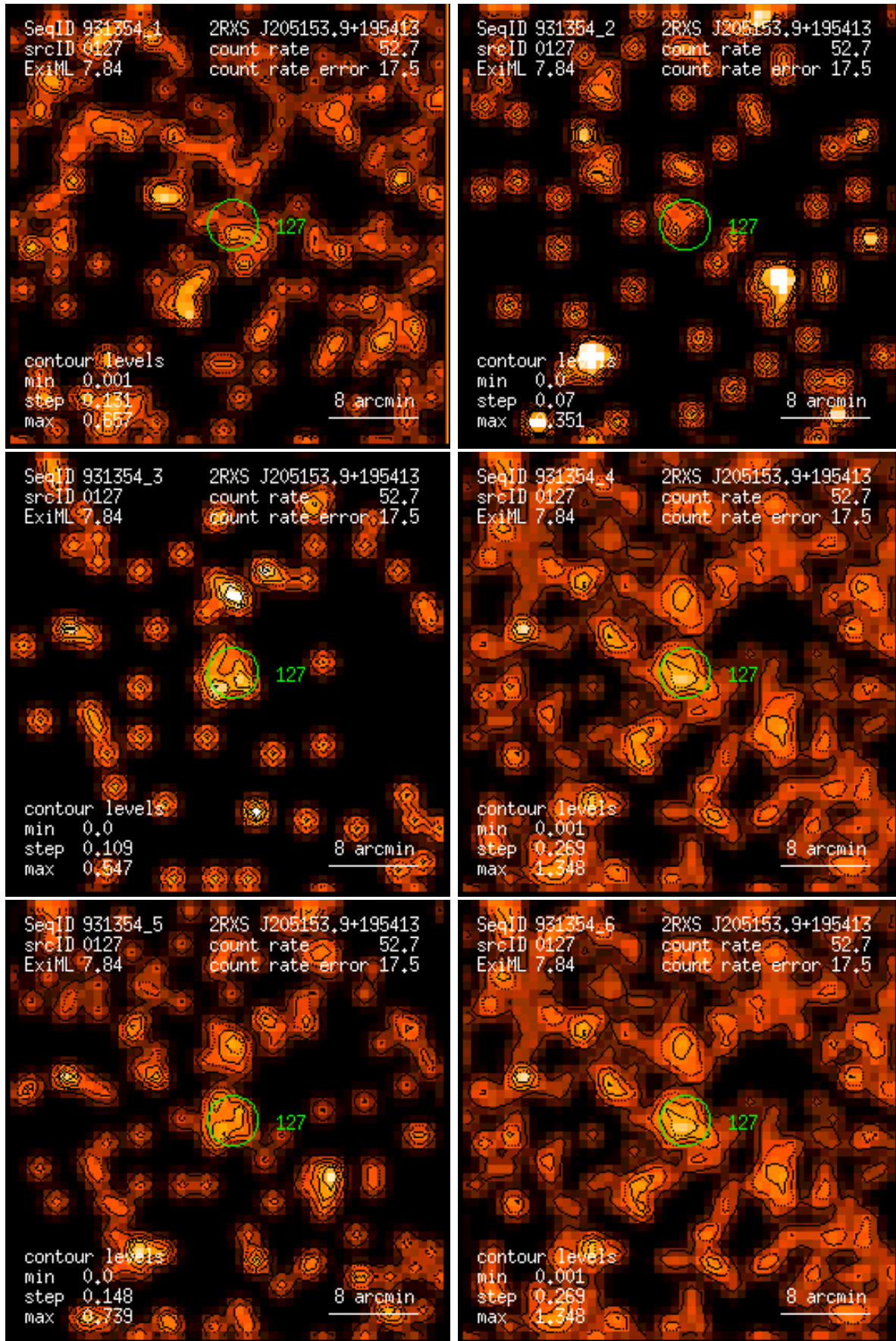
Figure 127: RASS 931354: detection 0127: band rate images, Gaussian filter: (1) PSPC channels 11 – 41, (2) 52 – 90, (3) 91 – 201, (4) 11 – 235, (5) 52 – 201, (6) 11 – 201. Broad band rates in counts/ks. Band rate contour levels in counts/ks/arcmin 2 .
