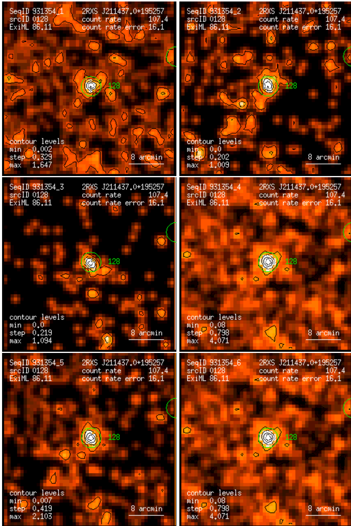
Figure 128: RASS 931354: detection 0128: band rate images, Gaussian filter: (1) PSPC channels 11 – 41, (2) 52 – 90, (3) 91 – 201, (4) 11 – 235, (5) 52 – 201, (6) 11 – 201. Broad band rates in counts/ks. Band rate contour levels in counts/ks/arcmin 2 .
